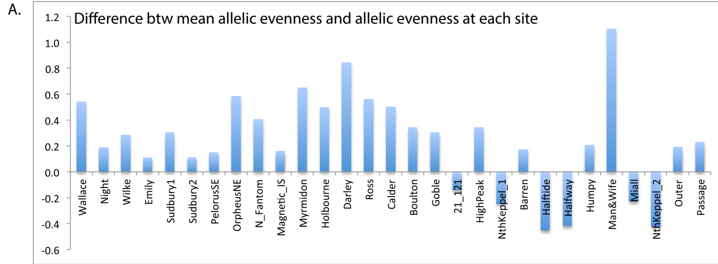
Fig. S1: Genetic diversity in A. millepora populations across the GBR: Difference between mean allelic evenness and allelic evenness at each site (A), and mean allelic evenness at each site (B).
