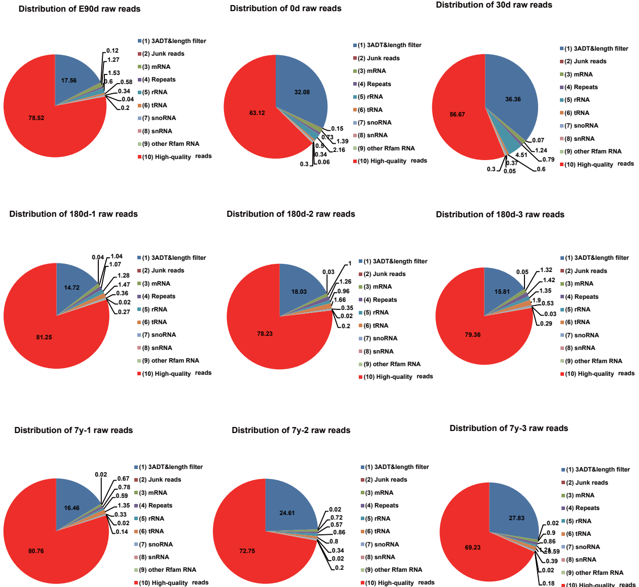
Figure S2 Distribution of raw reads in each library after applying a series of filters.
