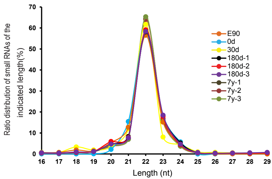
Figure S3 Length distribution of mappable reads.
