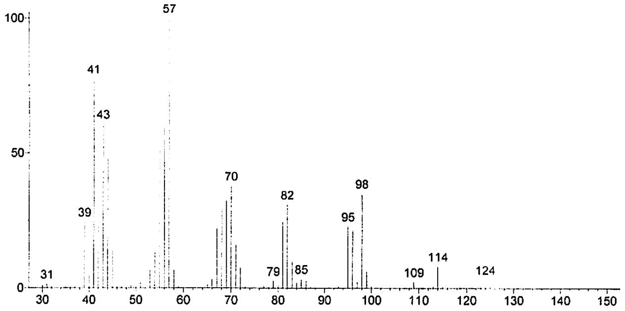
(Text File) Scan 690 (11.290 min): JA021209-2.D
