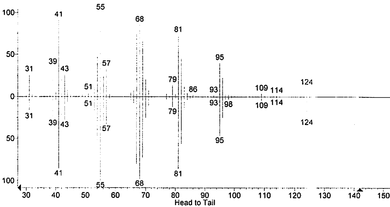
(Text File) Scan 758 (12.001 min): JA021209-2.D
