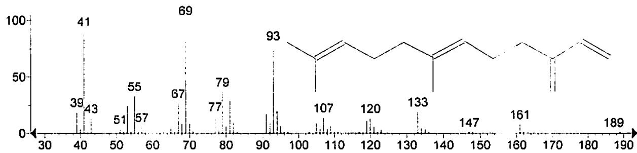
(replib) 1,6,10-Dodecatriene, 7,11-dimethyl-3-methylene-, (E)-
