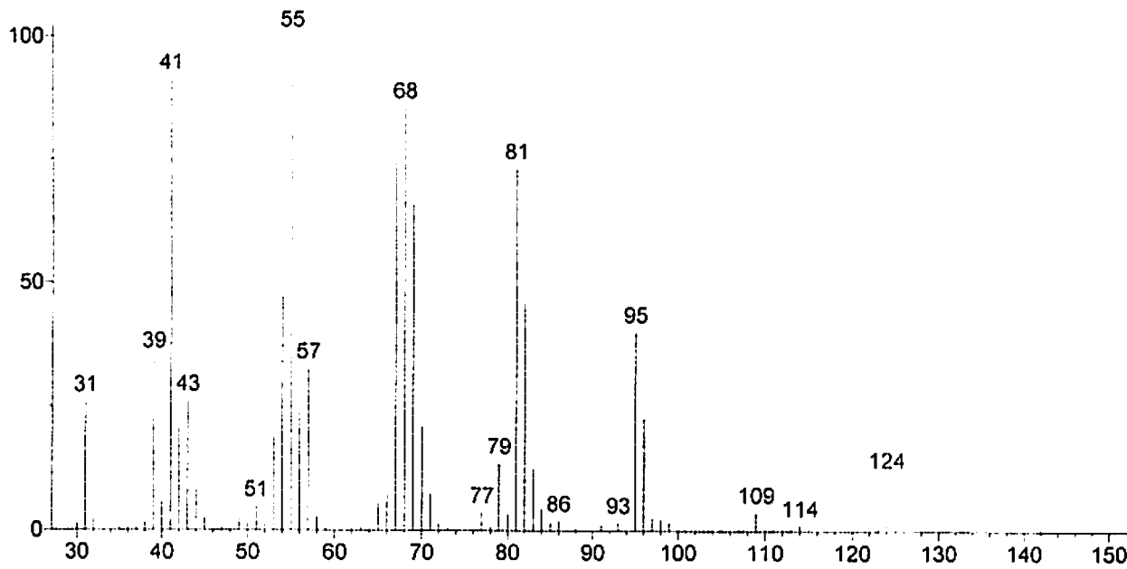
(Text File) Scan 758 (12.001 min): JA021209-2.D
