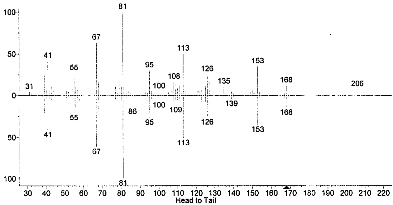
(Text File) Scan 1294 (17.606 min): JA021209-2.D (-1289)
