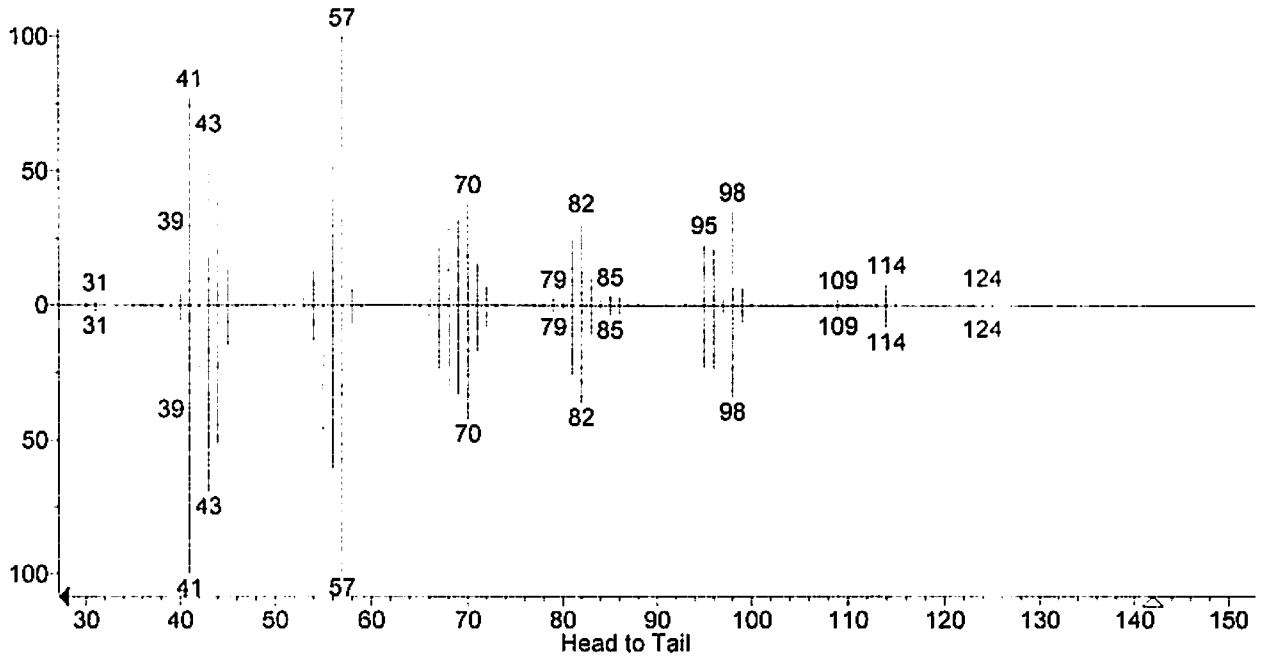
(Text File) Scan 690 (11.290 min): JA021209-2.D
