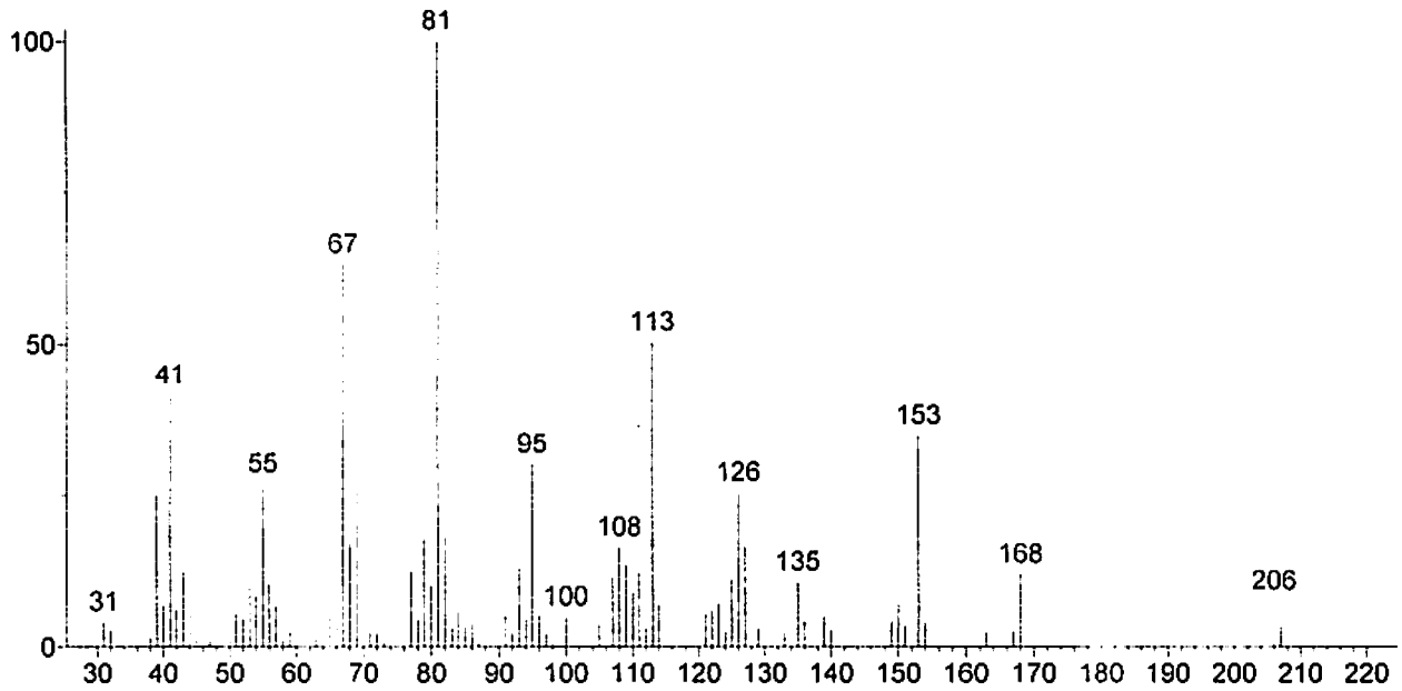
(Text File) Scan 1294 (17.606 min): JA021209-2.D (-1289)
