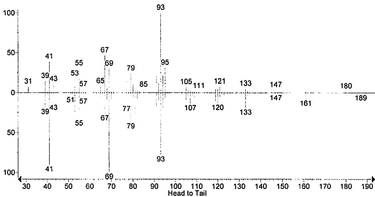
(Text File) Scan 1186 (16.477 min): JA021209-2.D (-1177)
