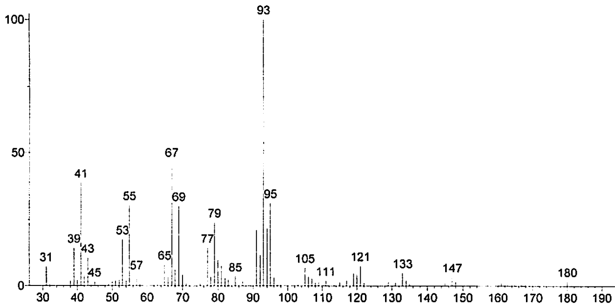
(Text File) Scan 1186 (16.477 min): JA021209-2.D (-1177)
