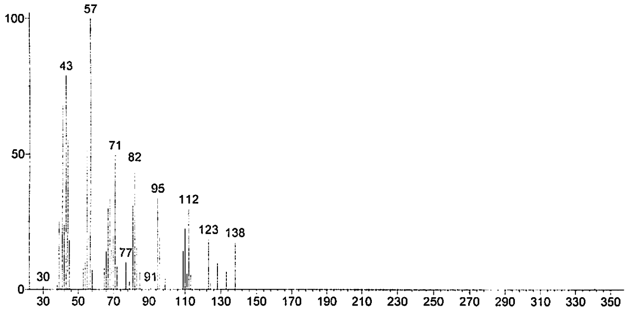
(Text File) Scan 852 (12.984 min): JA021209-2.D (-842)
