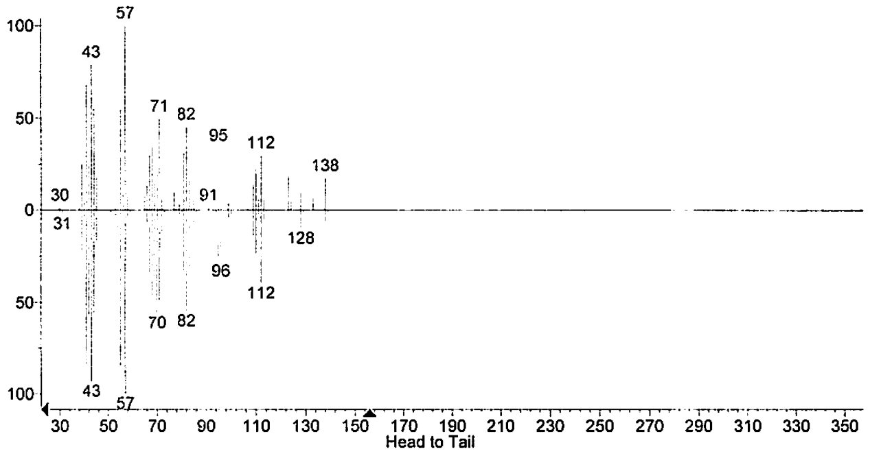
(Text File) Scan 852 (12.984 min): JA021209-2.D (-842)
