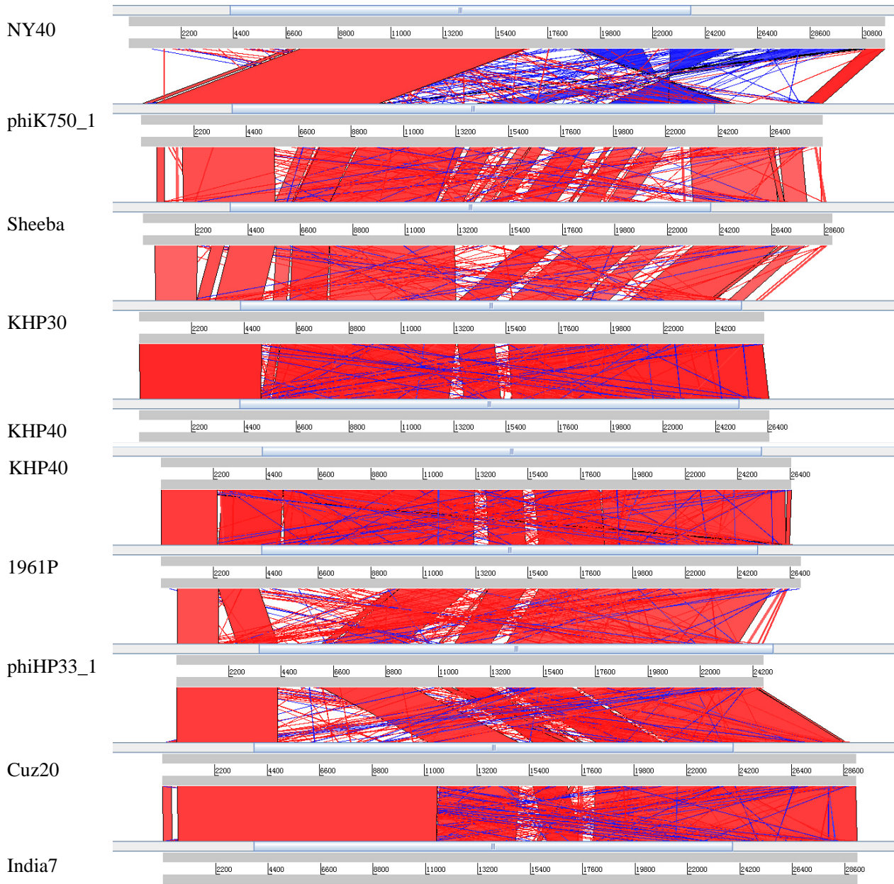
Figure S1. Comparative genomic analyses of clusterA1 phages of Helicobacter
