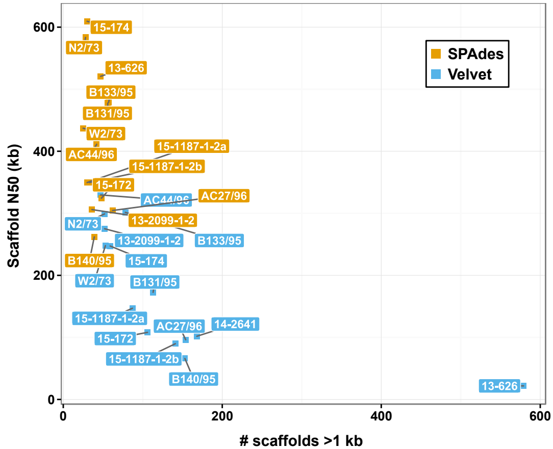
Supplemental Figure 2. The SPAdes assembler produces high quality assemblies. Genome sequences assembled using Velvet v. 1.2.10 (blue) and SPAdes v. 3.7.0 (orange) were compared based on scaffold N50 and number of scaffolds greater than 1kb in size.
