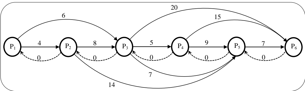
(B) Temporal pattern graph G(TP) with 0-edges
