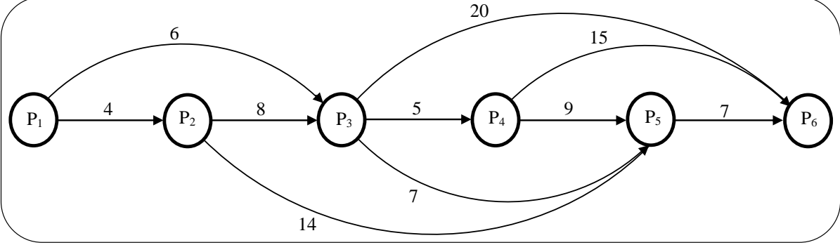
(A) A temporal pattern graph G(TP) with the given temporal pattern
