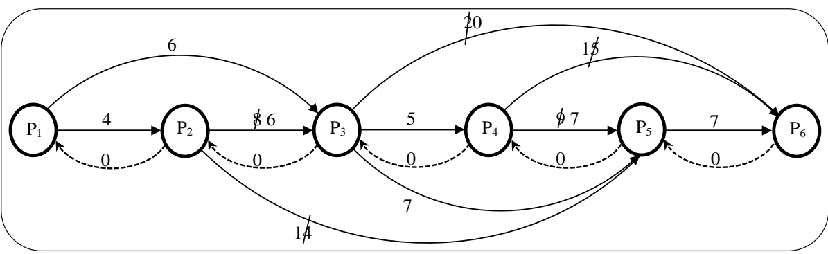
(C) Preprocessing phase of graph G(TP) with 0-edges
