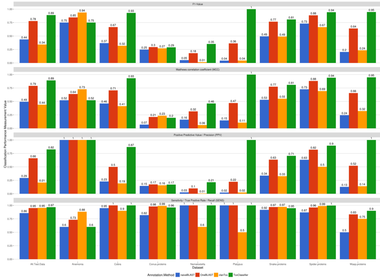
Figure S3/B Shows comparison of F1-Value (F1) , MCC score (MCC) , Positive Prediction Value (PPV) and Sensitivity (SENS) metrics for all test datasets and all tested annotation models (Naive-BLAST showed in blue, OneBLAST in red, ClanTox animal toxin prediction server in orange and ToxClassifier in green).
