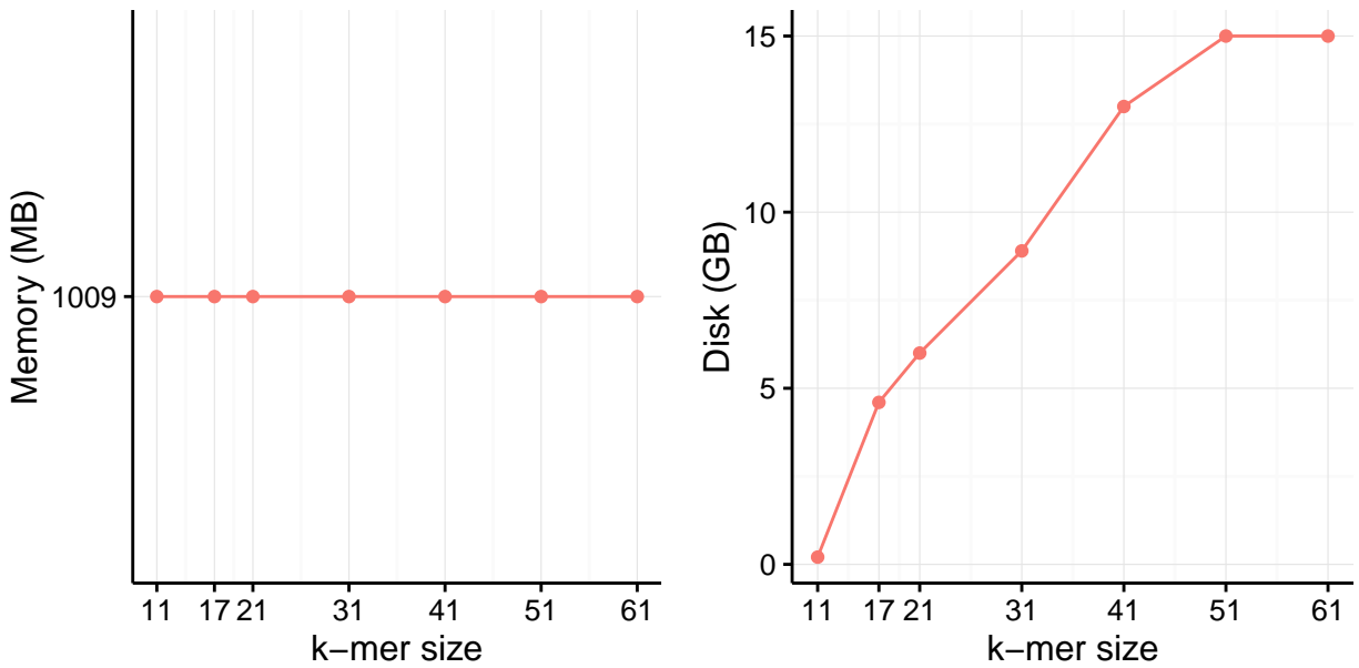
Supplementary Figure 1. Impact of the k-mer size on the performances of Simka. In each test above, Simka computed all the distances using the first 1M paired reads of 20 HMP samples on a single core. When k increases, the disk usage increases sub-linearly whereas the computation time and the memory usage stay constant.
