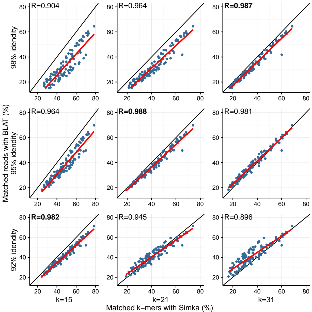
Supplementary Figure 2. Correlation between Simka and BLAT results. Each row corresponds to a BLAT identity threshold and each column to a k -mer size used by Simka. The value R is the Spearman correlation between Simka and BLAT results. Correlation values in bold are the greatest for each identity threshold.
