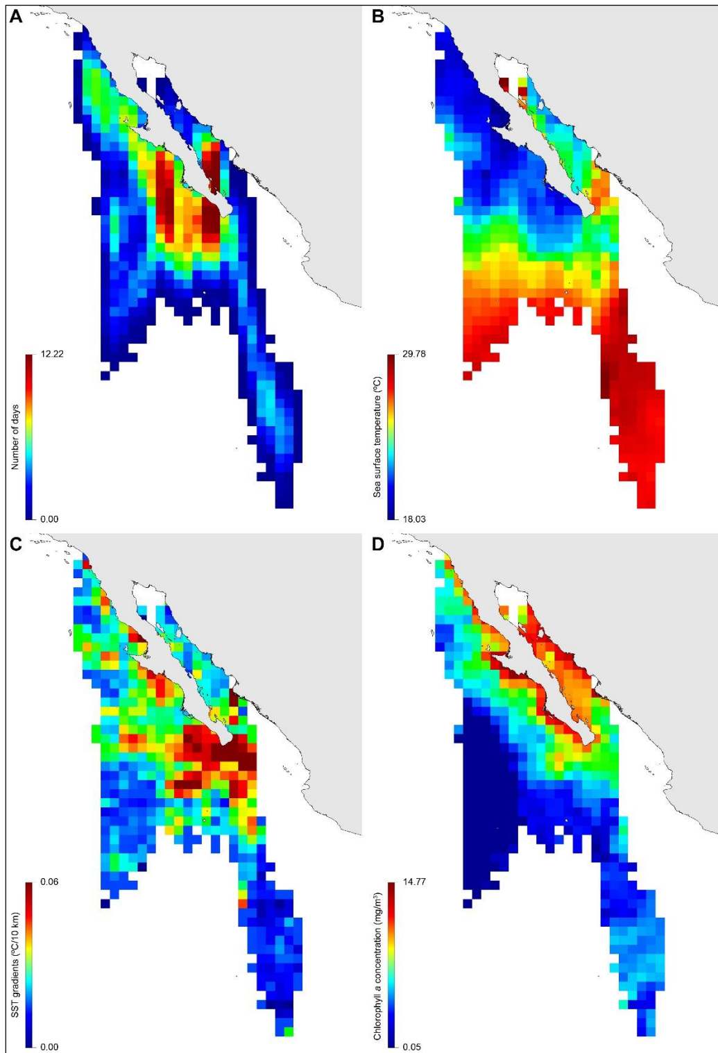
Figure S3 Averaged (0.5° grid) point density data (A) and environmental data (B-D); B – sea surface temperature (°C); C – sea surface temperature gradients (°C/10 km); D – chlorophyll a concentration. Note: these were the input data for the GLMM model.
