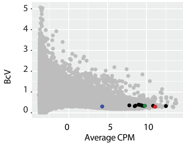
B) Biological Coefficient of Variation (BcV) against Average CPM
