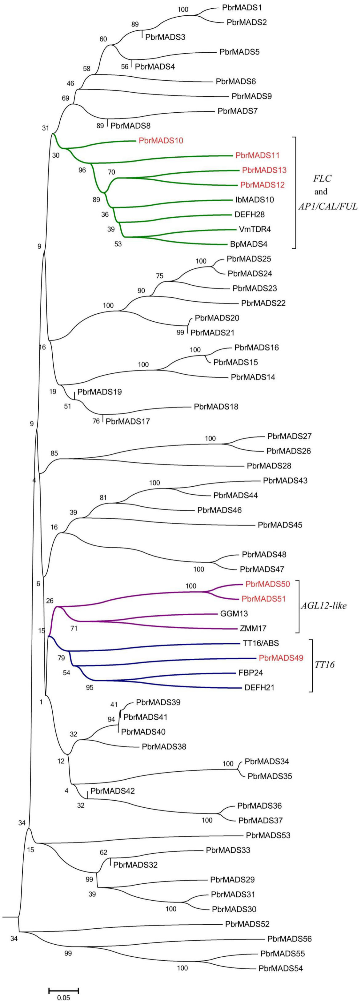
Supplementary figure 6. Phylogenetic tree of anthocyanin biosynthesis-related genes and type II PbrMADS genes. The tree was constructed using MEGA6.
