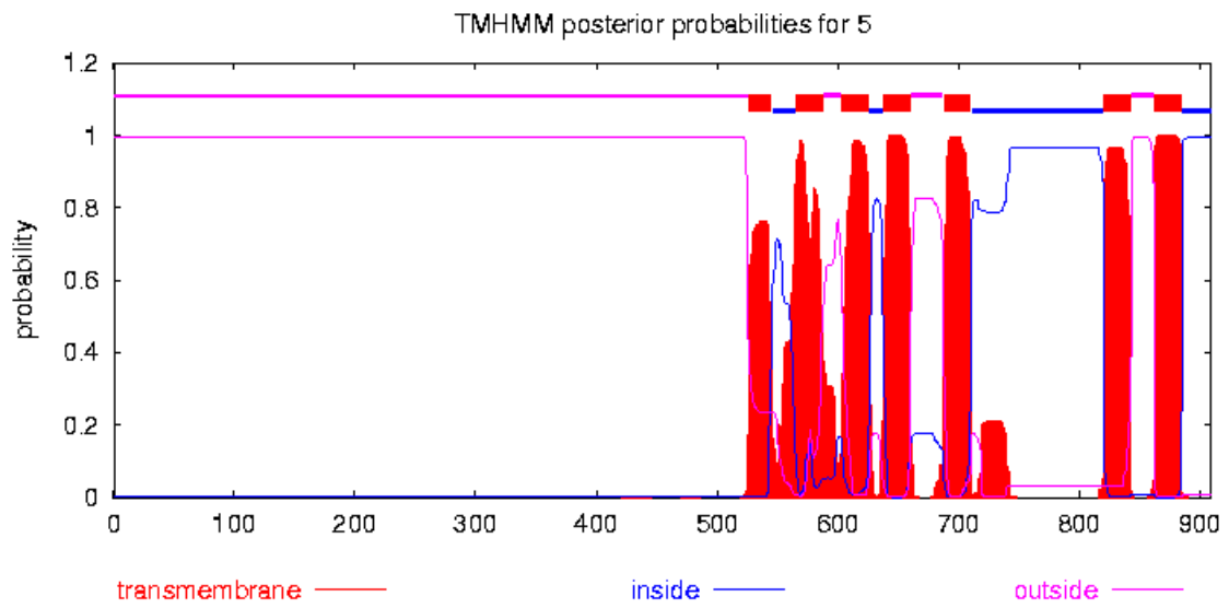
SF1 b: Profile 2 of transmembrane topological organization of complete sequences of protein of CHSBasidio database.
