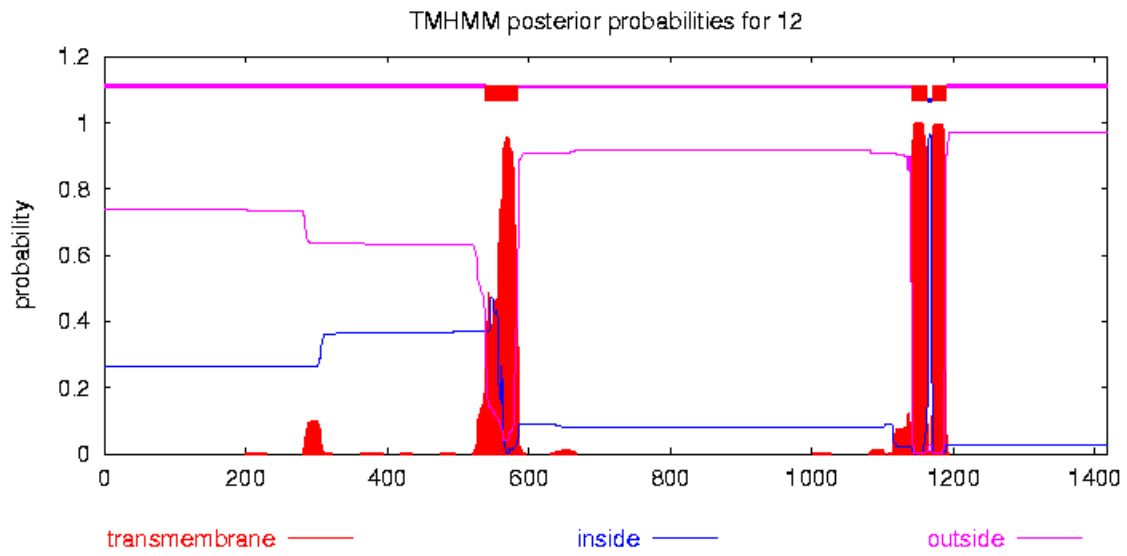
SF1 d: Profile 4 of transmembrane topological organization of complete sequences of protein of CHSBasidio database.
