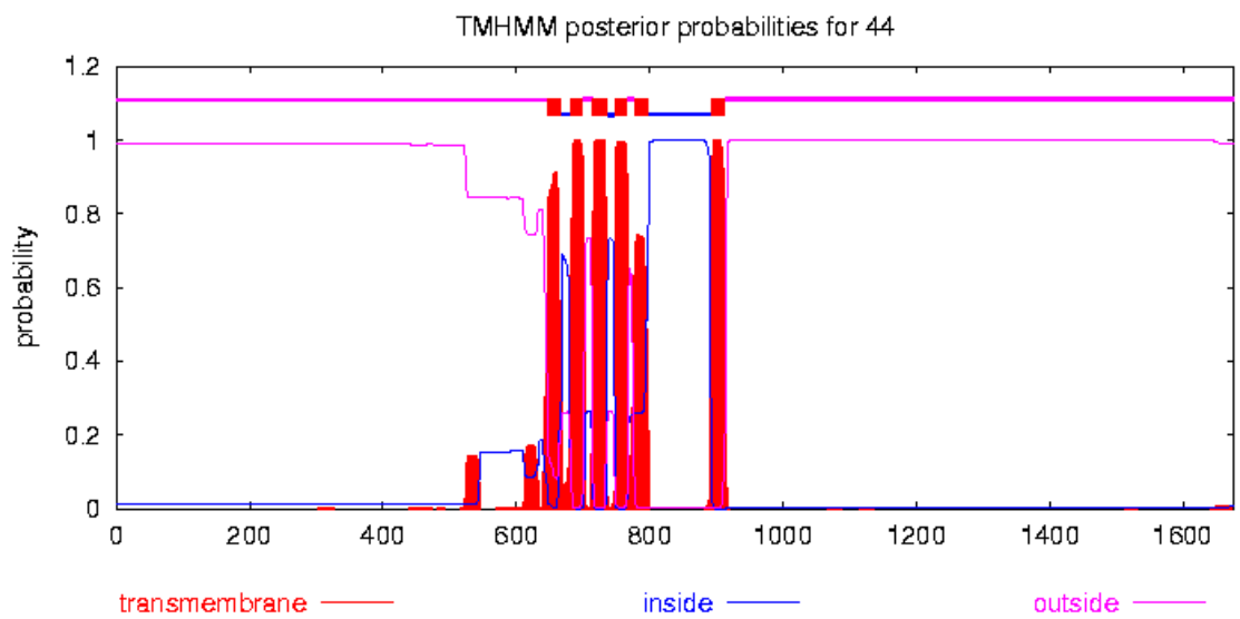
SF1 g: Profile 7 of transmembrane topological organization of complete sequences of protein of CHSBasidio database.
