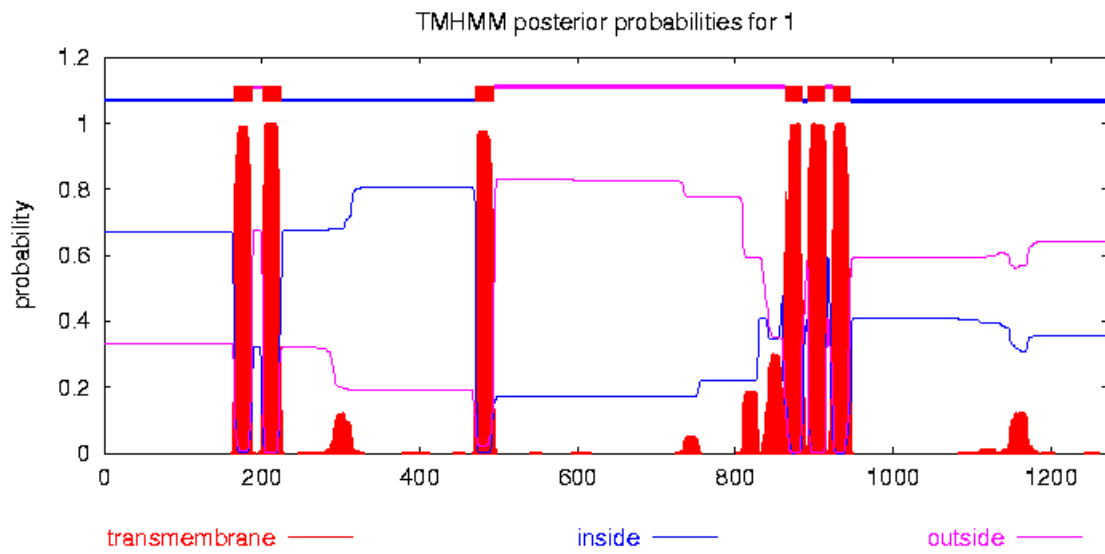
SF1 a: Profile 1 of transmembrane topological organization of complete sequences of protein of CHSBasidio database.
