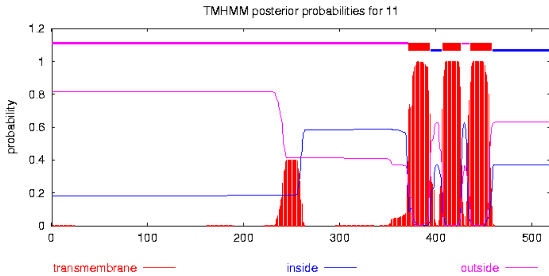
SF1 e: Profile 5 of transmembrane topological organization of complete sequences of protein of CHSBasidio database.
