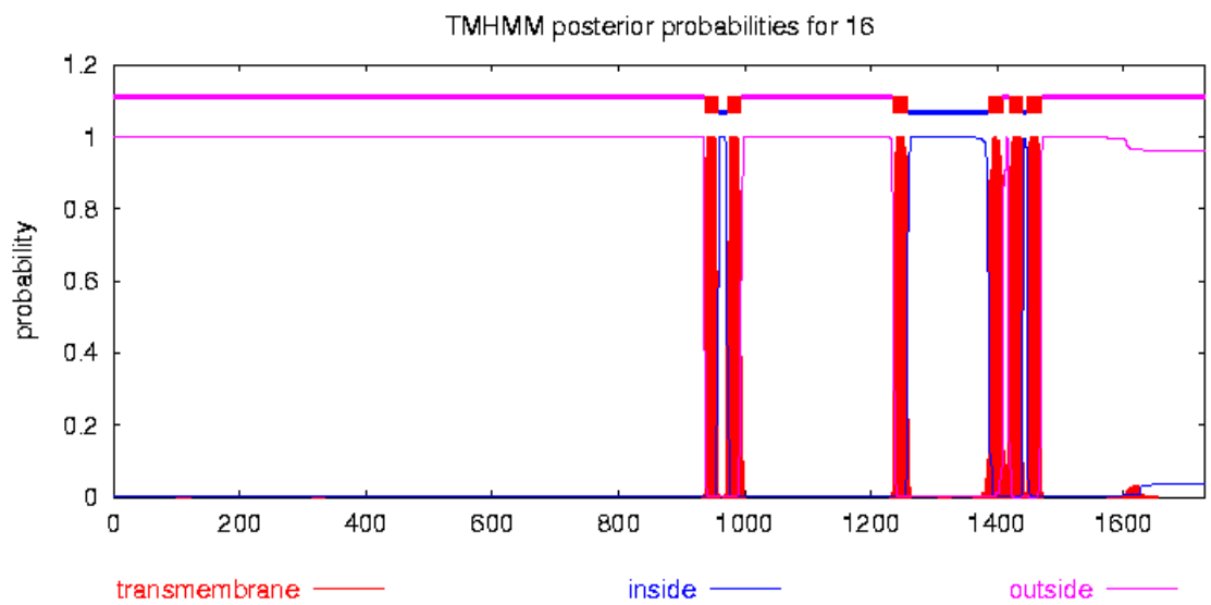
SF1 c: Profile 3 of transmembrane topological organization of complete sequences of protein of CHSBasidio database.
