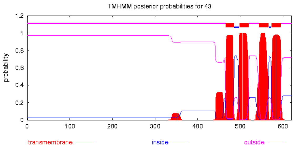
SF1 f: Profile 6 of transmembrane topological organization of complete sequences of protein of CHSBasidio database.
