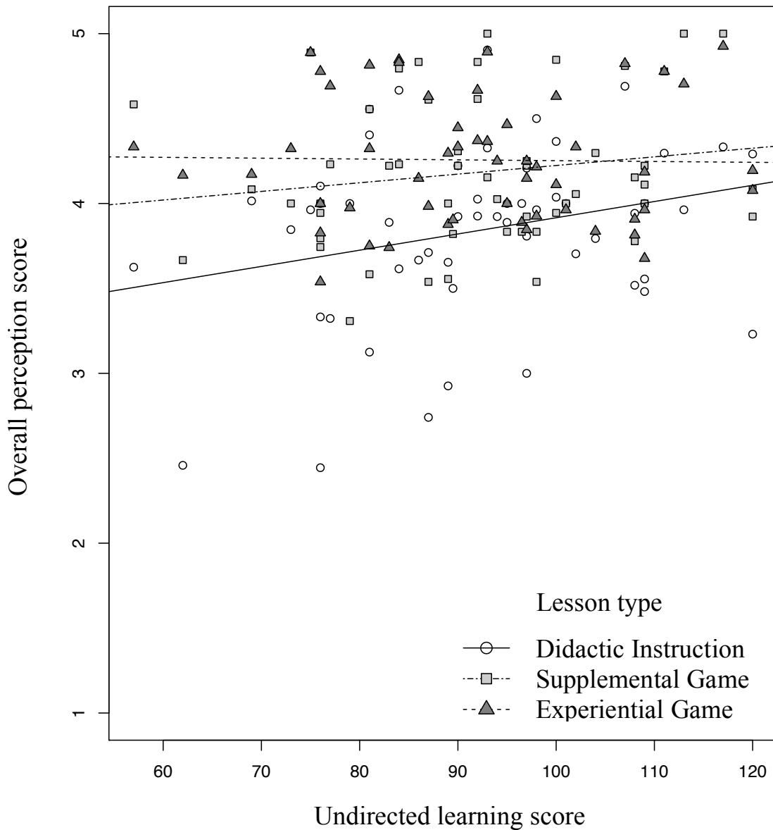
Figure S1. Figure showing relationship between overall perception score and undirected learning score. There was a significant interaction between lesson type and undirected learning score (General Linear Mixed Model models: \chi^2 = 7.29 , df = 2 , p = 0.026 ). The correlation coefficient for Didactic Instruction is 0.009, that for Supplemental Game is 0.005 and that for Experiential Game is 0.
