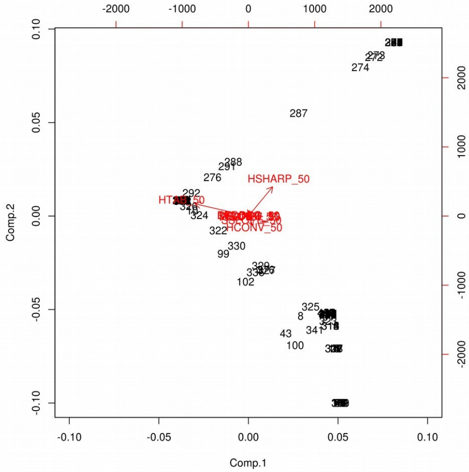
Figure S4: Plot showing the first two principal components of geomorphology variables (see Table S1 for full code legends).
