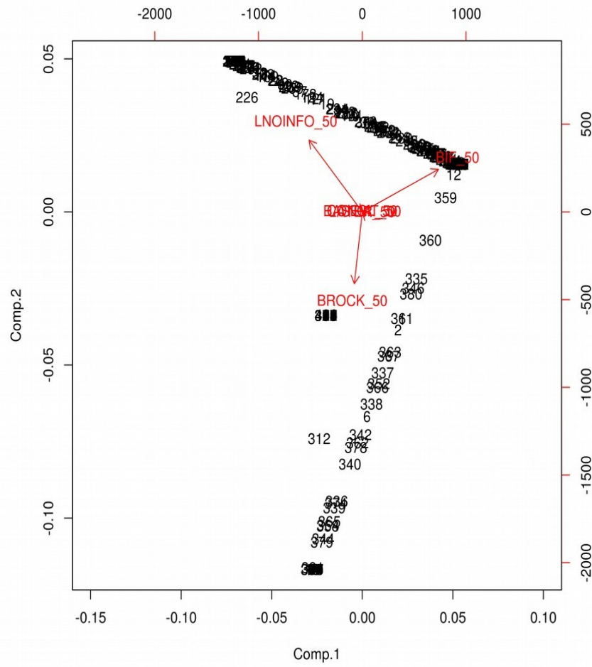
Figure S3: Plot showing the first two principal components of lithology variables (see Table S1 for full code legends).
