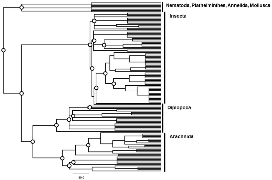
Figure S2: Phylogeny for the troglobitic species included in this study, retrieved from Hedges & Kumar (2009). Circles indicate dated nodes, while further nodes are evenly distributed among two dated nodes.
