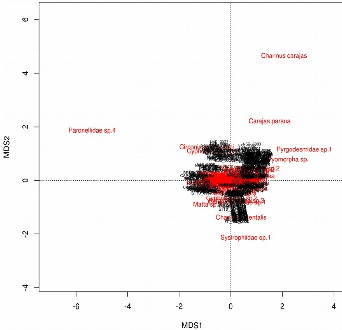
Figure S1: Principal coordinate analysis showing the distribution of some troglobitic species across the studied caves. Caves plotted in the same direction as specific troglobitic species actually contain those species.
