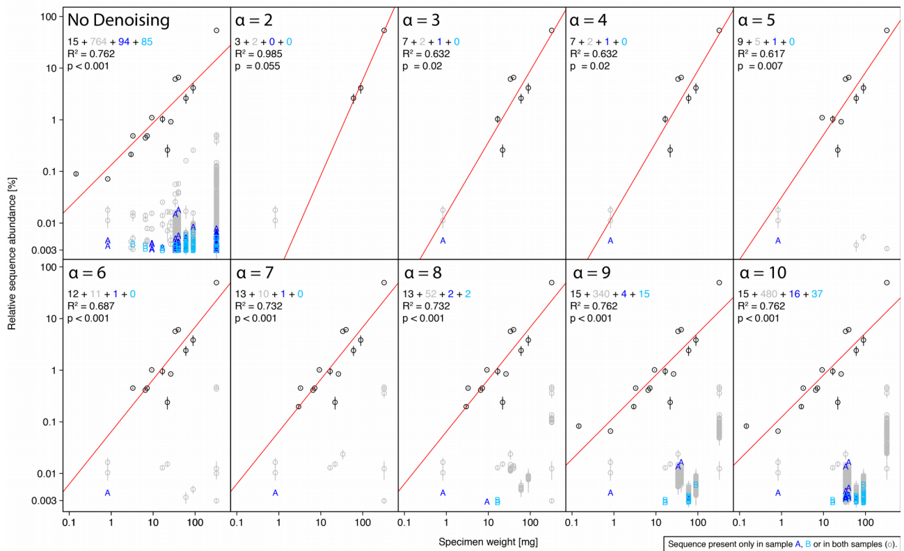
Figure S4: Effect of different haplotype recovery of in the single species mock sample, when using different alpha values with Unoise3 (as integrated in the JAMP package). Not all reads are shared between both replicates (indicated by A or B instead of a circle). The 15 expected haplotypes are shown in black, while unexpected ones are highlighted in gray or blue. Error bars show the standard deviation of relative read abundance between both replicates, for the respective haplotype.
