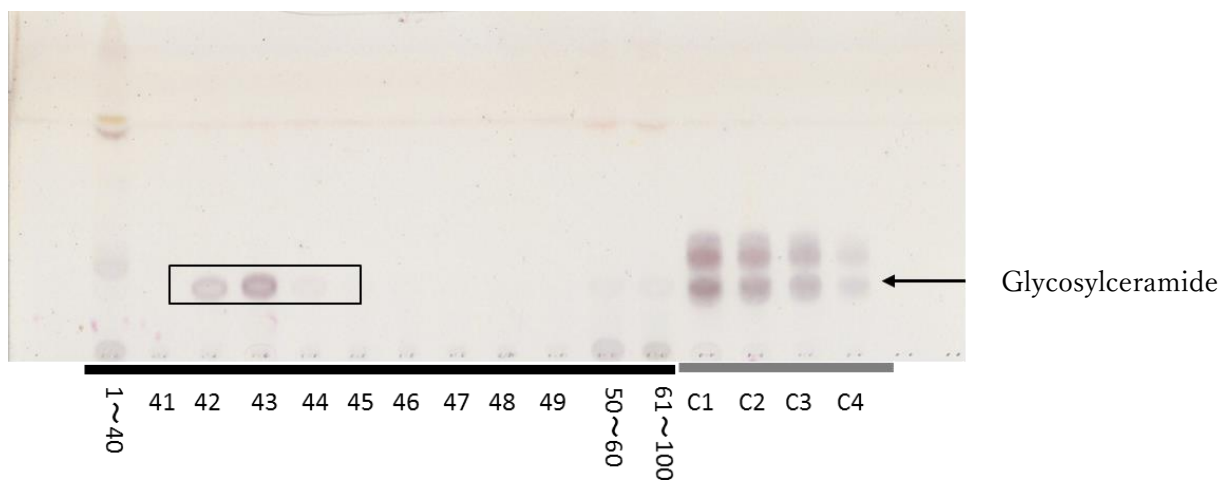
Fig. S1. Purification of glycosylceramide from mycelia of A. oryzae .
