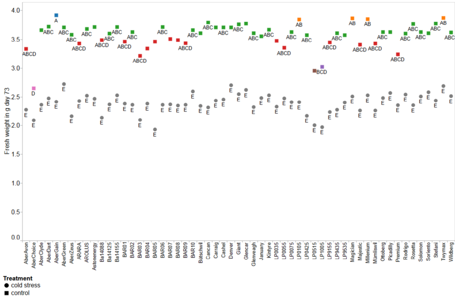
Supplemental Materials Figure 1: Fresh weight (g) at day 73 for the 57 accessions grown under cold stress and control conditions. The letters represent significant different groups according to an ANOVA test and a Tukey ranking test. Both accession and treatment were highly significant.
