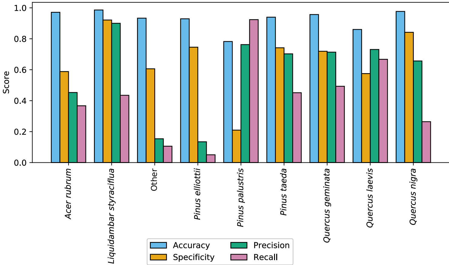
Model performance on test data using sample probabilities
