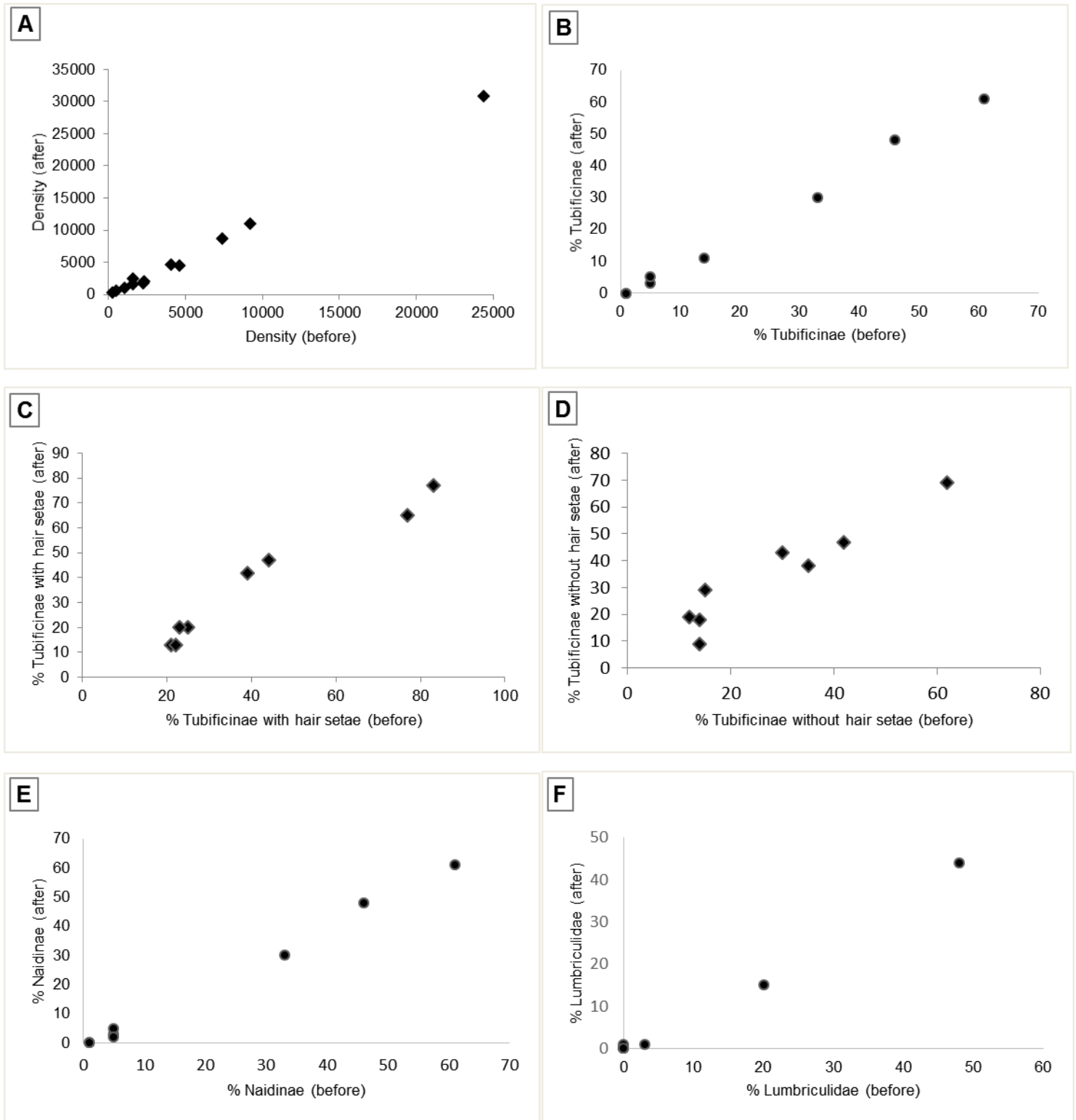
Supplemental Figure S1. Relationships between the percentages of oligochaete densities and families/subfamilies obtained before and after the addition of absolute ethanol to formalin-fixed oligochaete communities. Oligochaete densities per 0.1 m 2 (A), Tubificinae (B), Tubificinae with hair setae (C), Tubificinae without hair setae (D), Naidinae (E) and Lumbriculidae (F)
