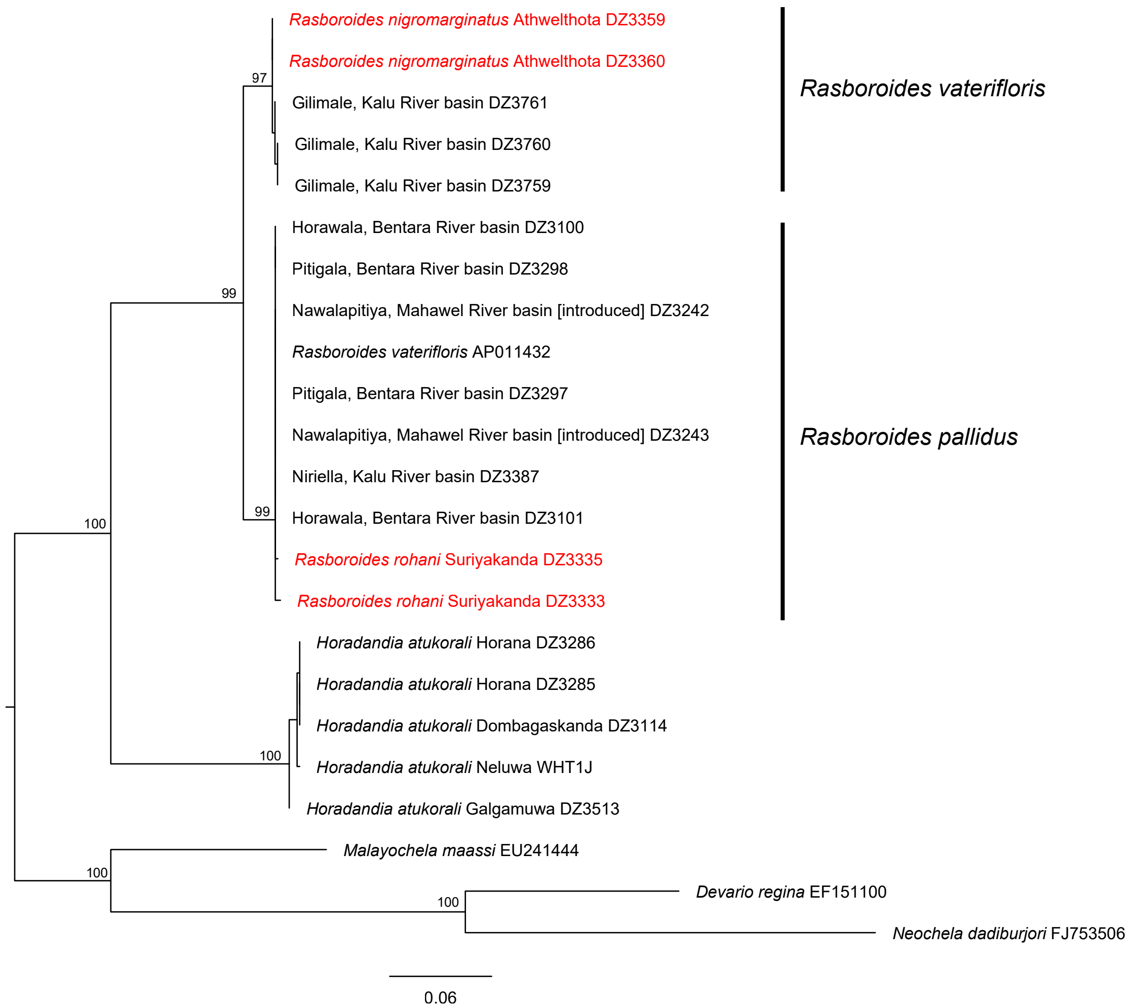
Supplement Figure 1. Maximum Likelihood phylograms based on A , cytb and B , coi datasets for species of Rasboroides in Sri Lanka. Numbers above nodes represent the ML bootstrap values. The scale bar represents number of changes per site.
