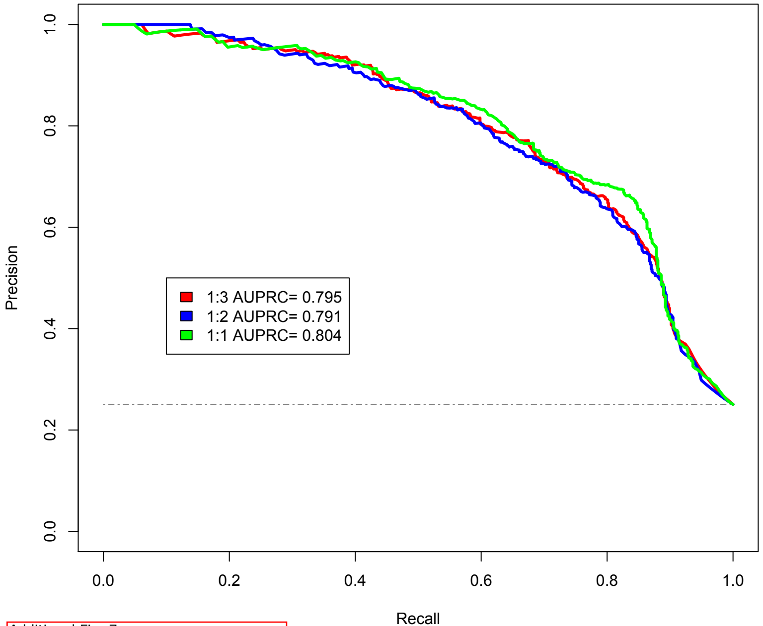
Lu et al's test dataset (14 Bacteria) - PR curve
