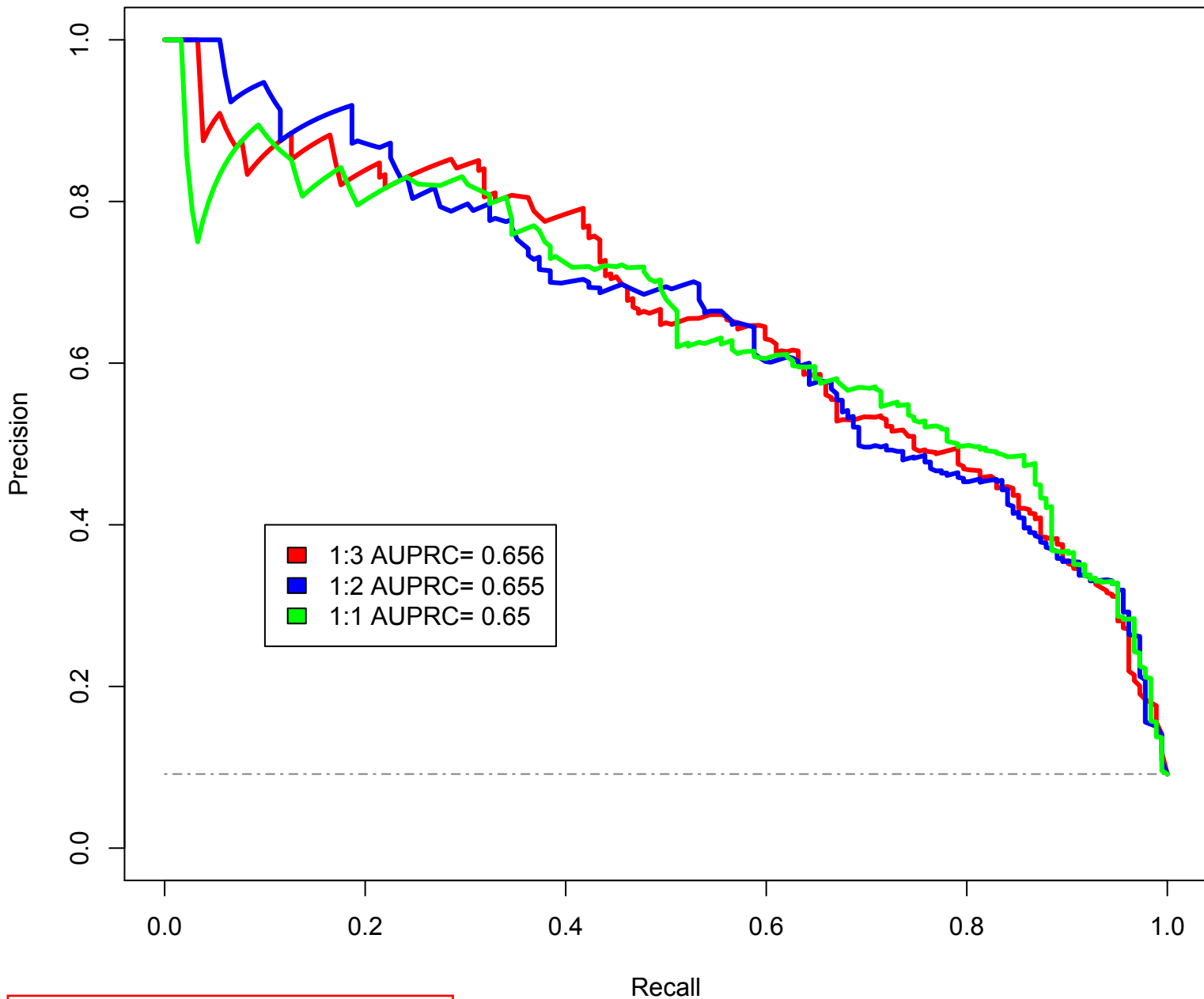
SLT2 test dataset - PR curve
