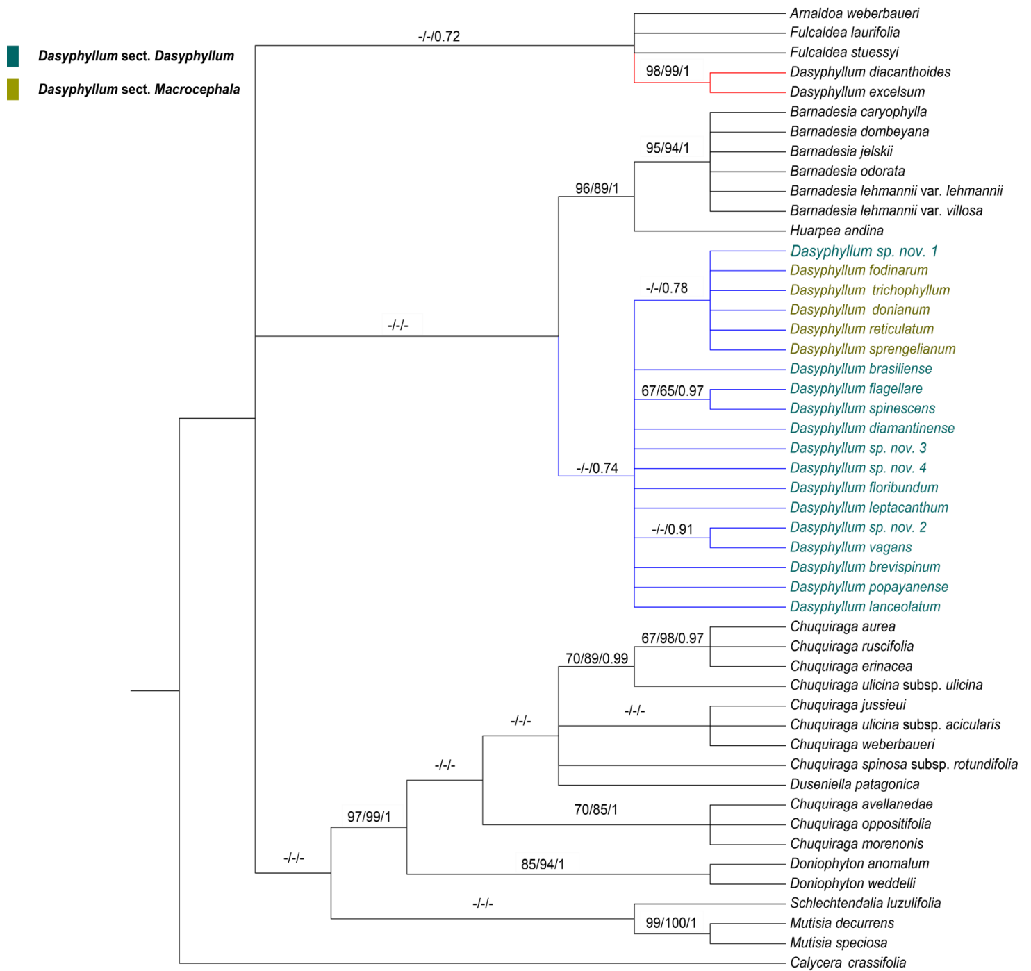
Phylogenetic relationships of Dasyphyllum based on psbA-trnH marker inferred from Bayesian inference. Support values are indicated above the branches in the order of parsimony, maximum likelihood, and Bayesian analyses. Support values lower than 63% are indicated by a dash (-).
