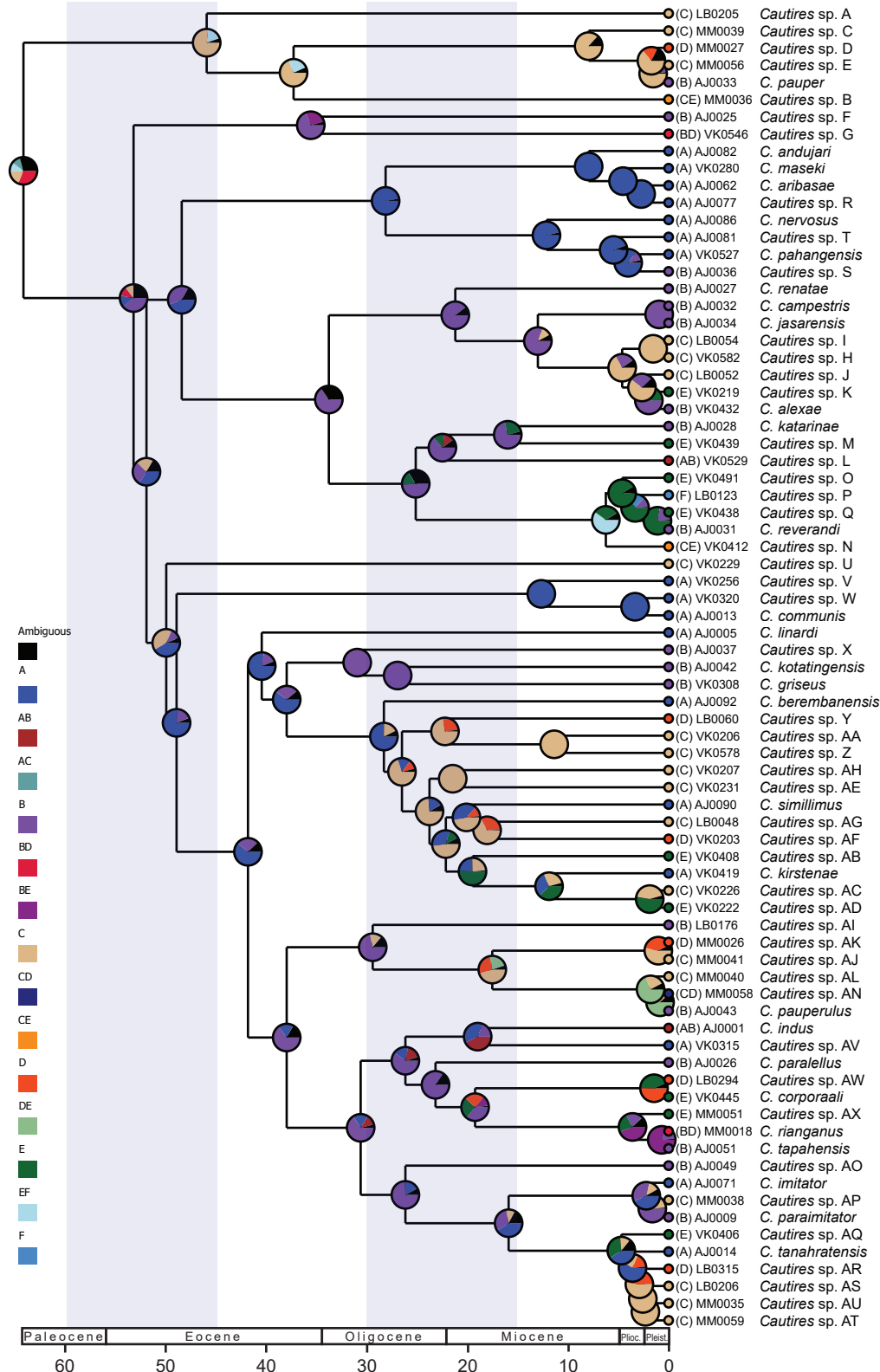
Supplementary Figure S3. Time calibrated maximum clade credibility tree of Cautires with reconstruction of specific geographic localities. Letters refer to sampled areas: (A) Malaysia: Cameron Highland, (B) Malaysia: lowlands, (C) Sumatra: Tuju, (D) Sumatra: Merapi, (E) Sumatra: Sibayak, (F) Java and their respective combinations.
