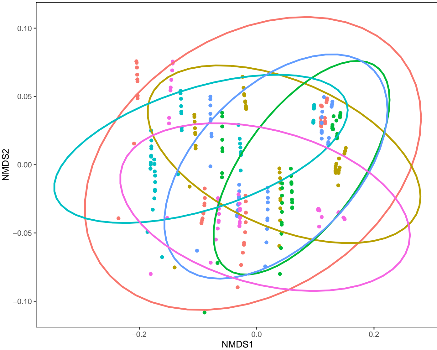
a) NMDS Plot for study years
