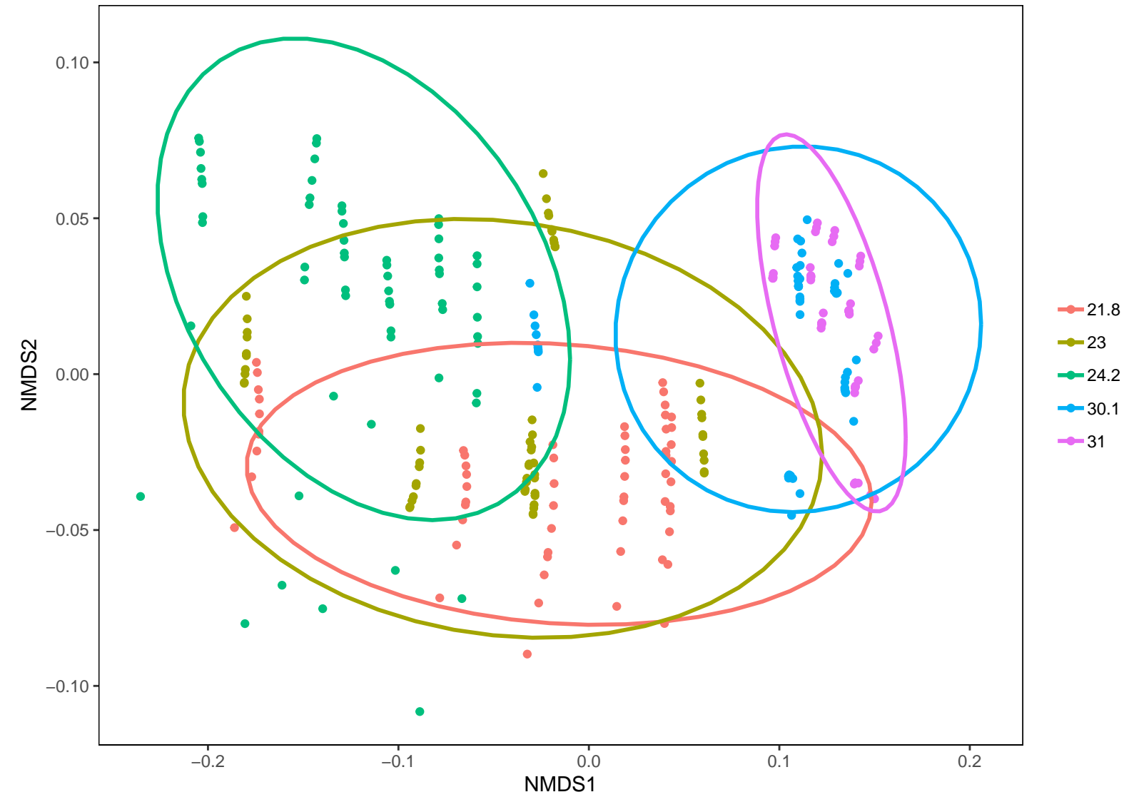
b) NMDS Plot for Continental Index
