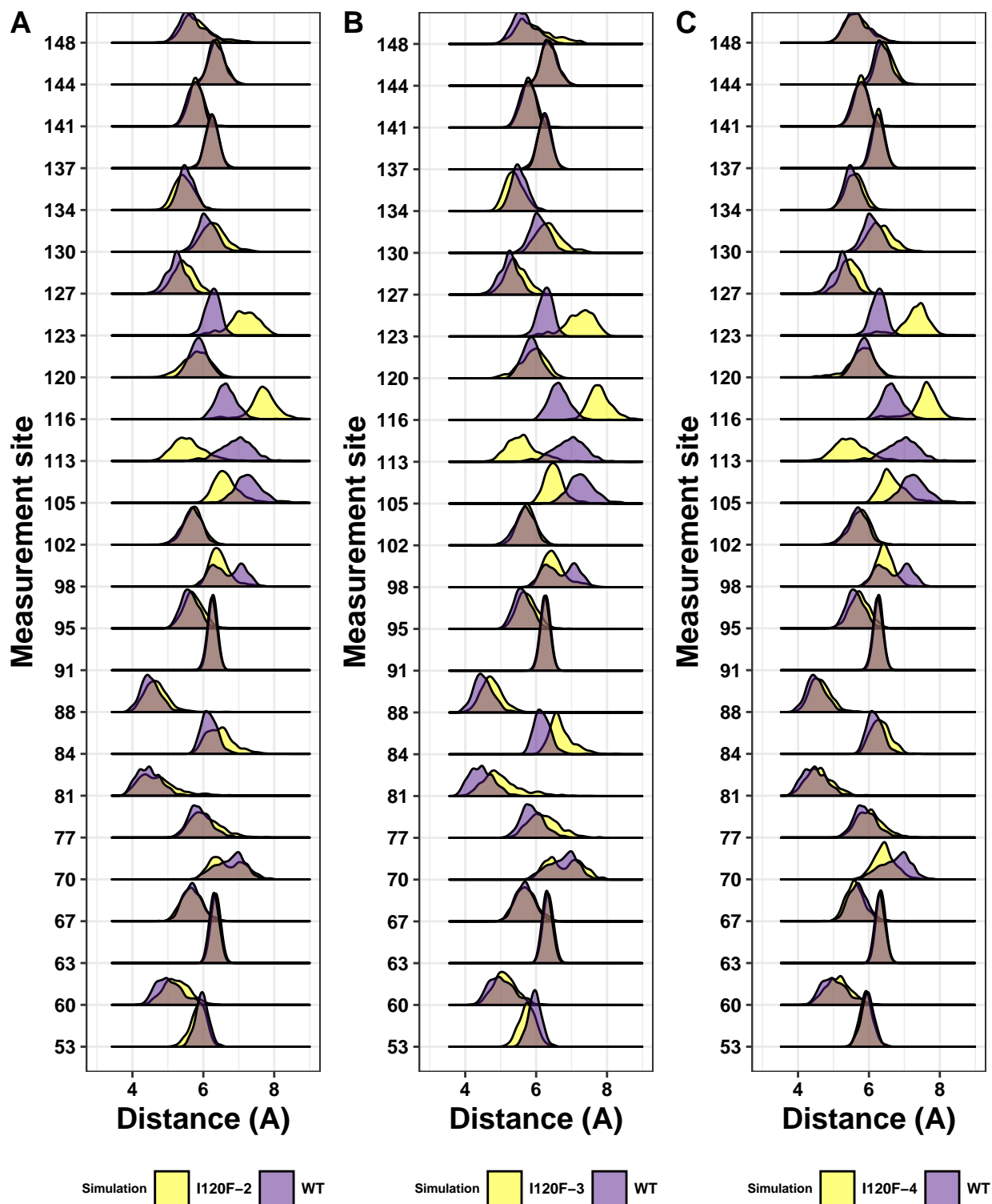
Figure 2: Differences in side chain position between the wild-type Isoleucine (purple) and the mutation Phenylalanine (yellow) for the 3 replicate simulations. Ile120Phe simulation (yellow) and the wild-type simulation (purple). Overlap is shown in grey
