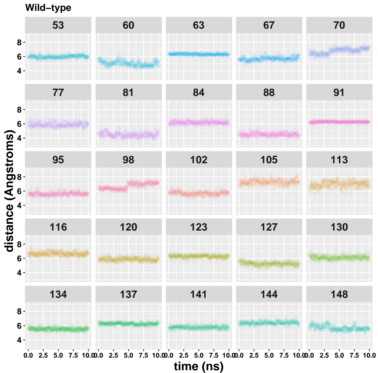
Figure 3A: Distance between amino acids at the designated position plotted over the simulation time.
