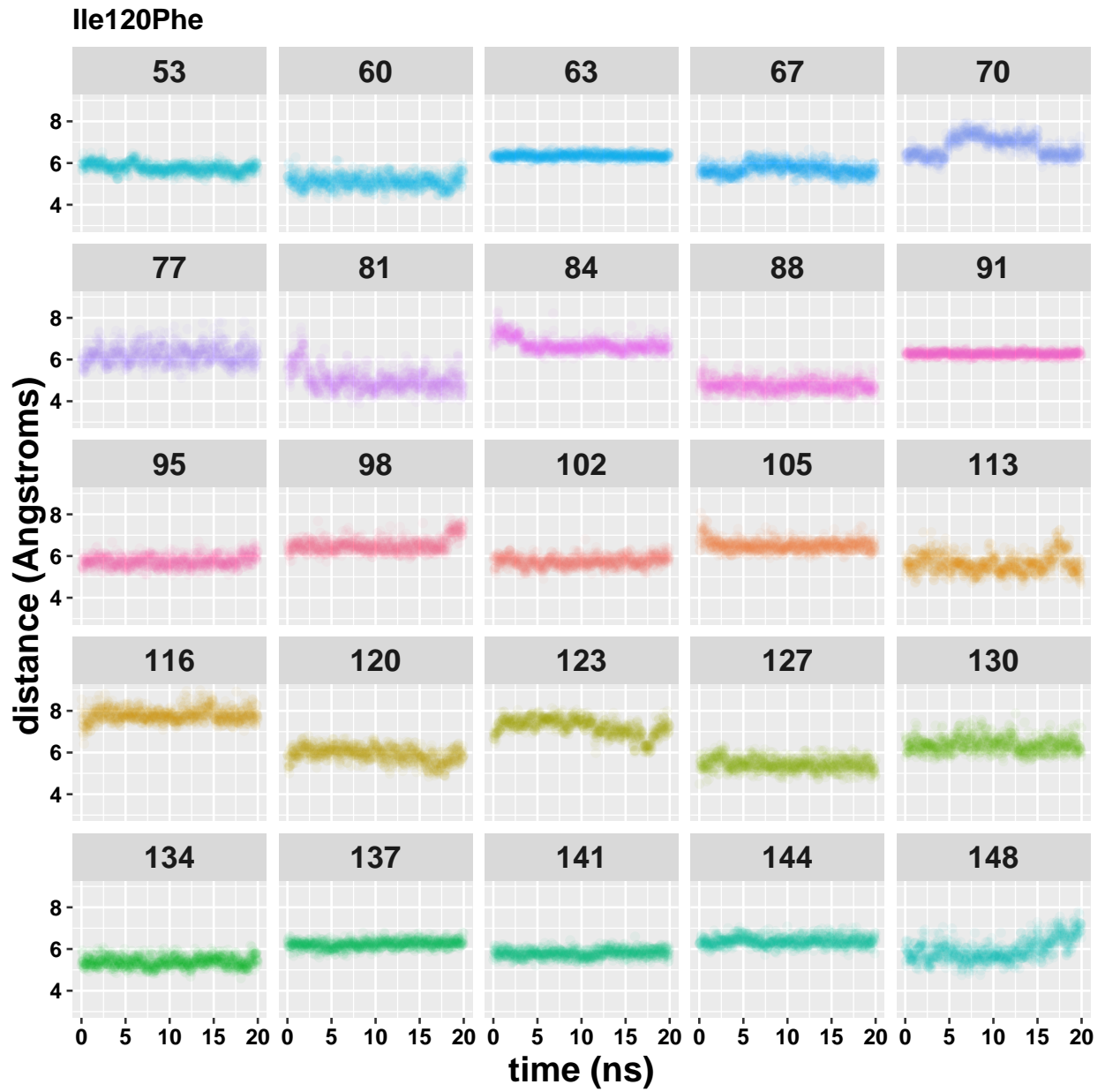
Figure 3B: Distance between amino acids at the designated position plotted over the simulation time for Tetherin with an I120F mutation.
