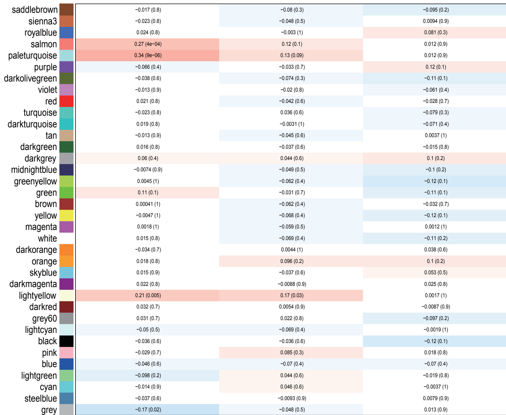
(A) BLCA.Module-trait relationships
