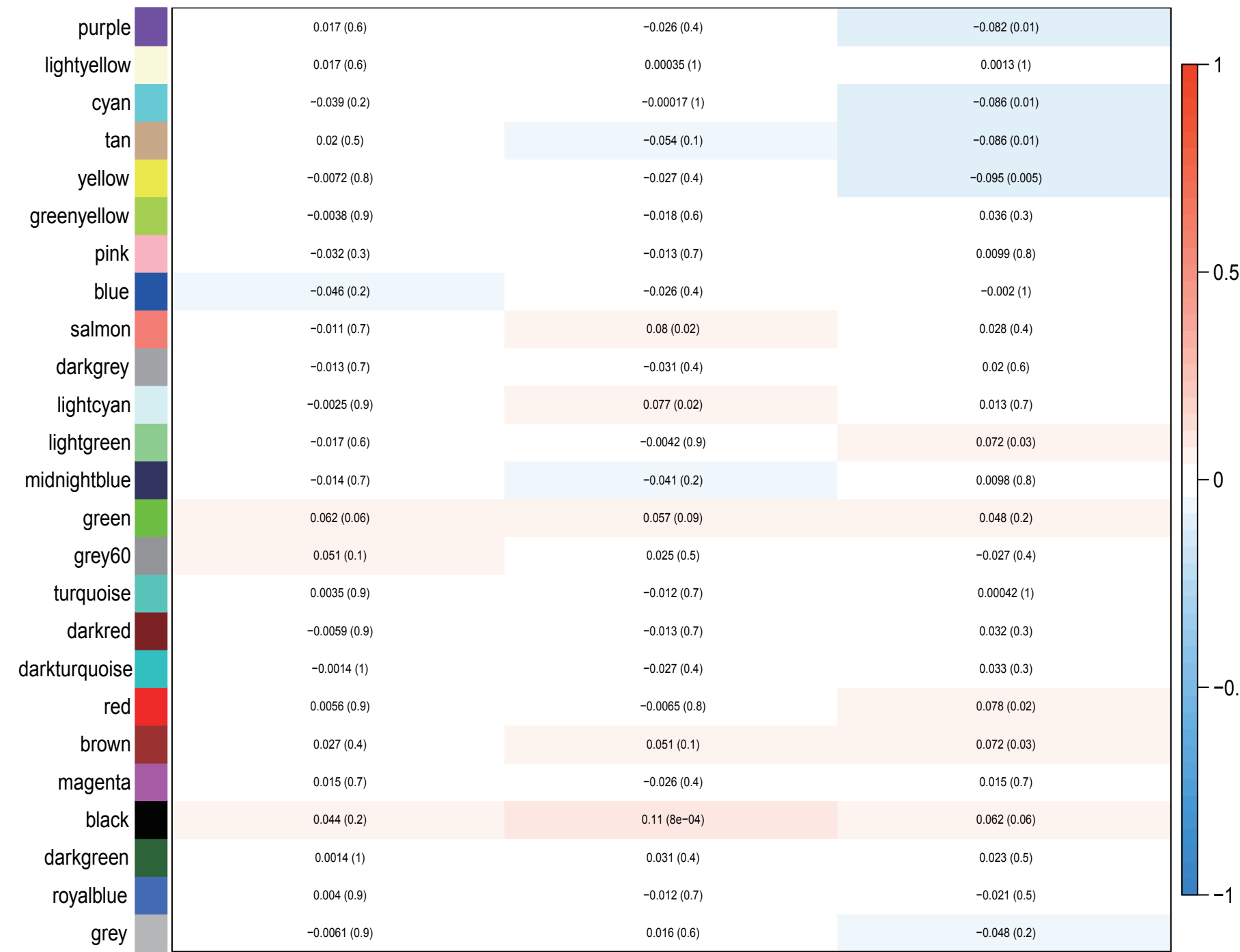
(B) BRCA.Module-trait relationships
