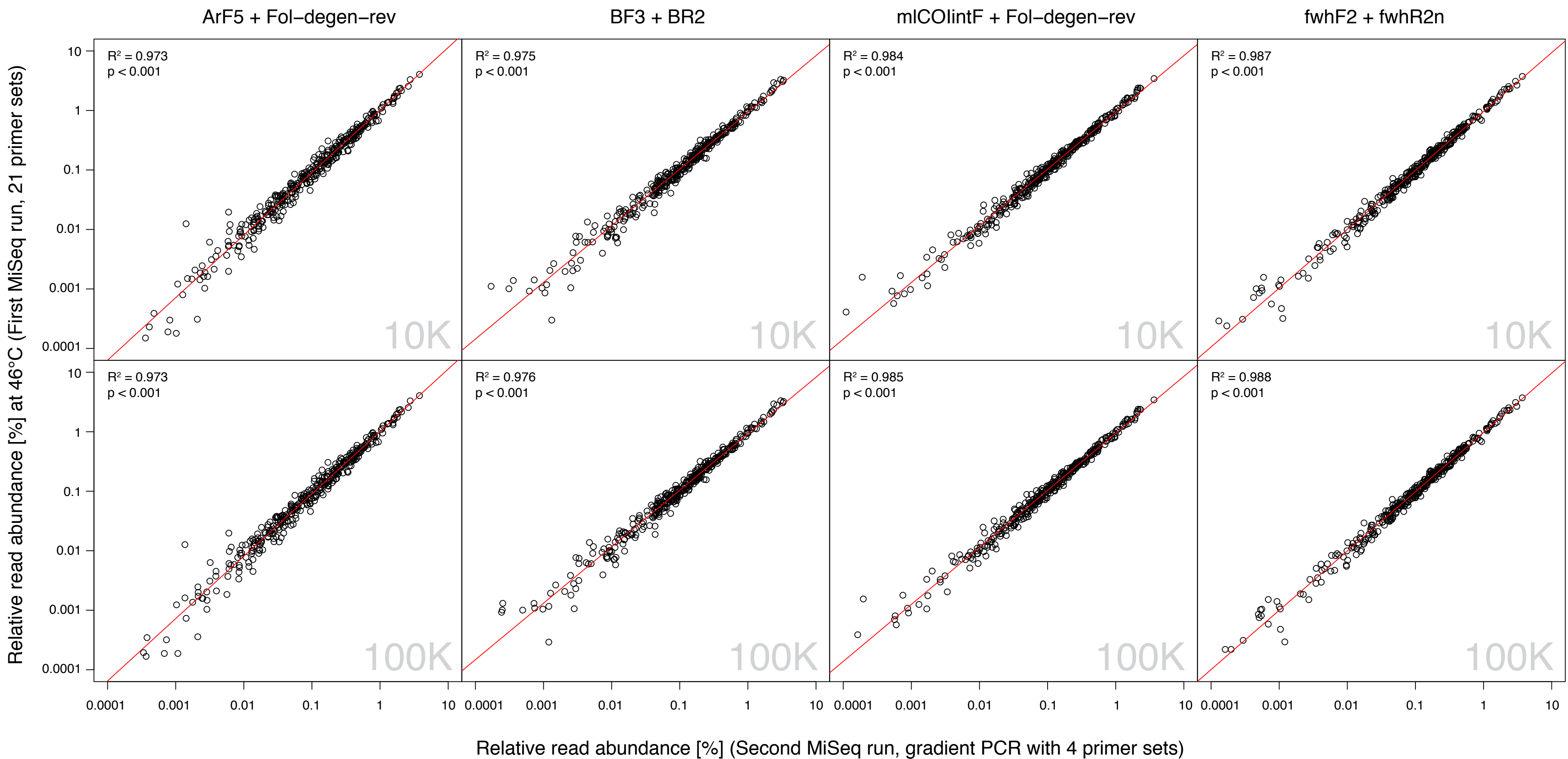
Figure S15: Comparison of read abundances of the 4 primer sets tested in both the mock sample primer test and gradient PCR run (both at 46°C). Sequencing depth was subsamples to 10,000 or 100,000 sequences with 1000 replicates. The red line indicates the linear regression between both samples.
