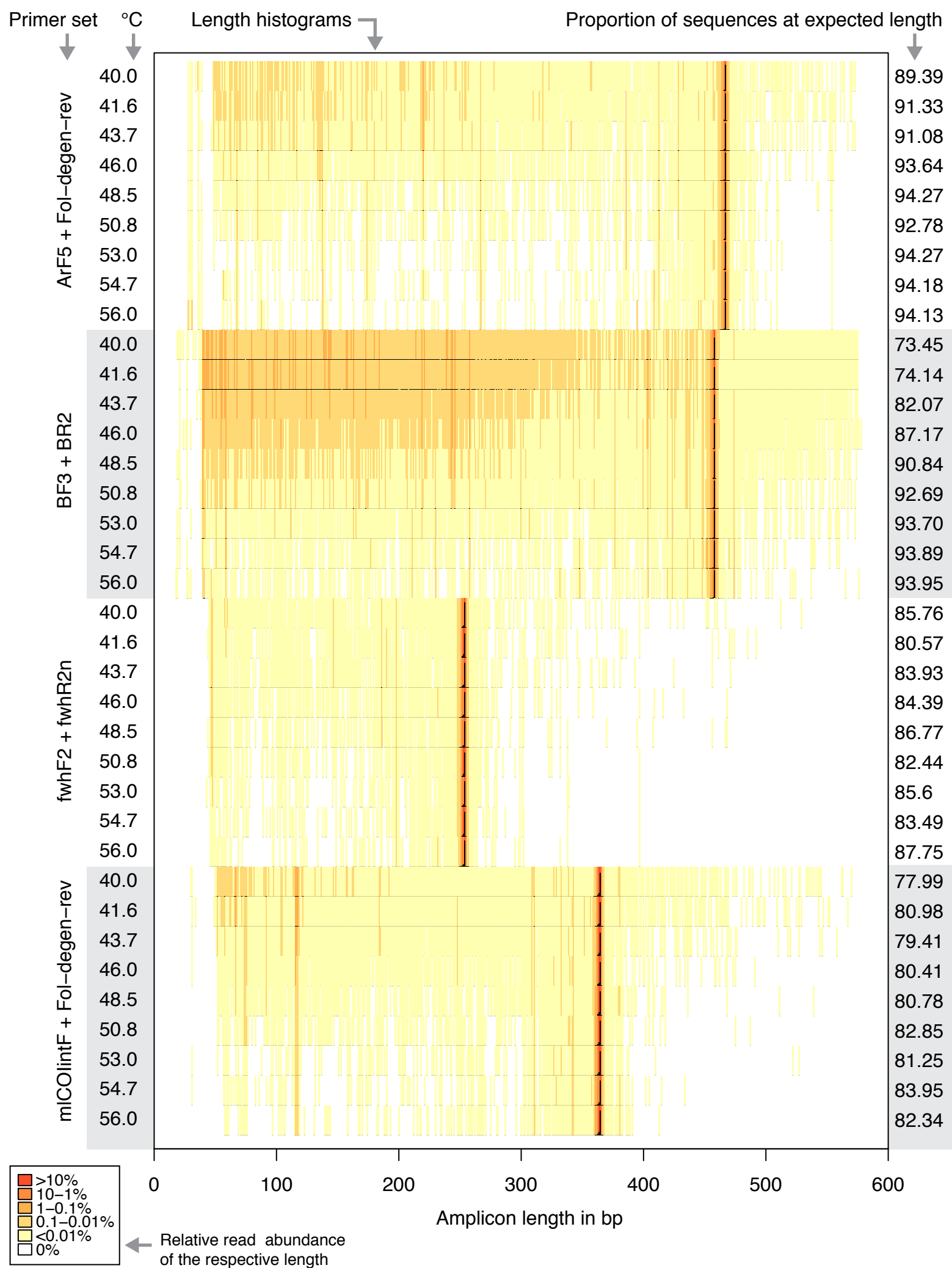
Figure S17: Histograms showing read length for four primer sets amplifying the mock sample in a gradient PCR (no primer trimming, 40-56°C). The number on the right indicates the proportion of sequences that have the exact expected amplicon length. In addition to black bars in the histogram, relative read abundance is also indicated with different shading.
