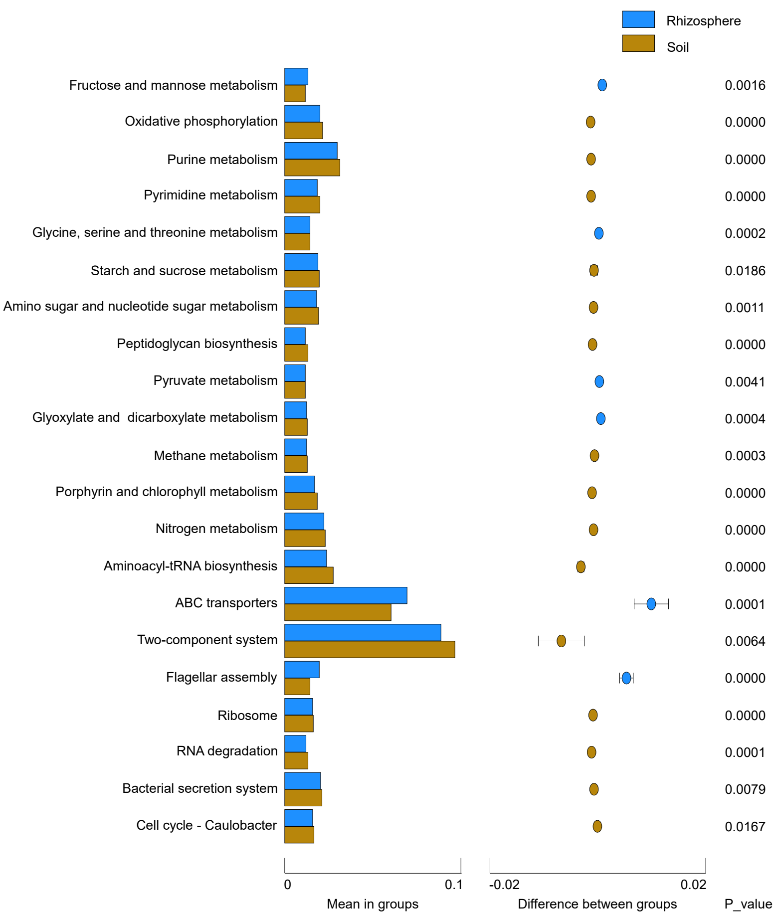
Figure S10. KEGG functional analysis in bacteria. Bars in the left, mean values of KEGG enrichment. Bars across circles, 95% confidence interval of the differences. Center of circles, differences of the mean values. Numbers in the right, p values of the significance test.
