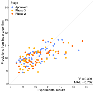
(a) HIC
