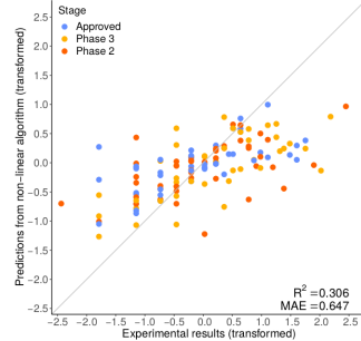
(c) CIC
