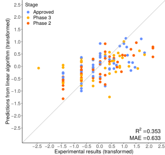
(b) SMAC
