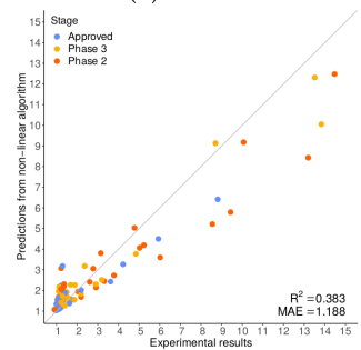
(e) ELISA
