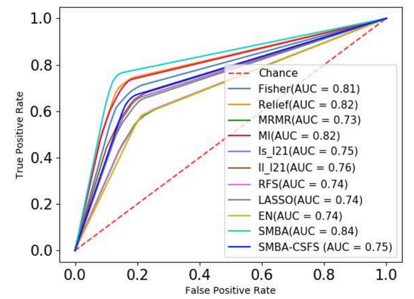
(c) CLL_SUB_111 (3)
