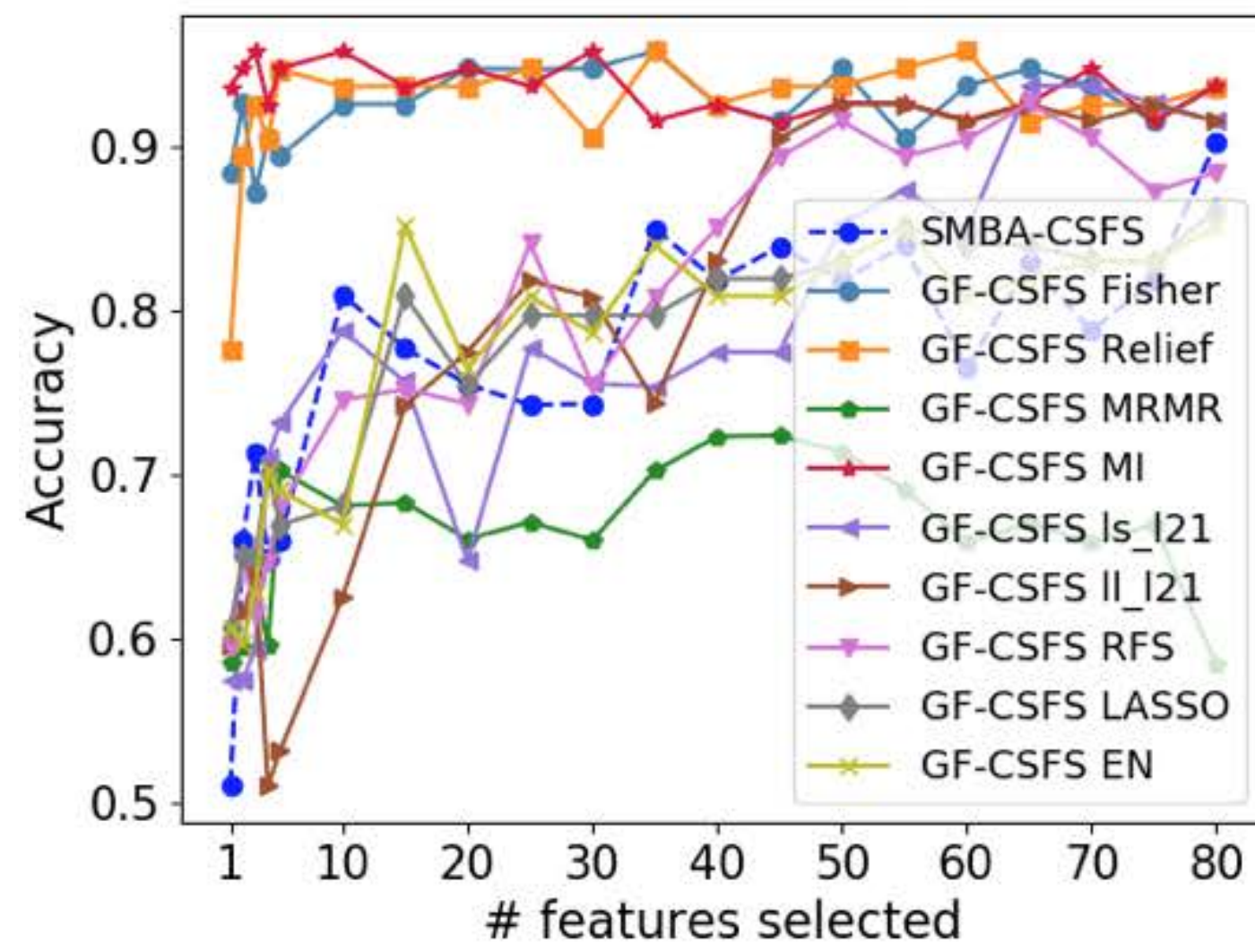
(a) ALLAML (2)
