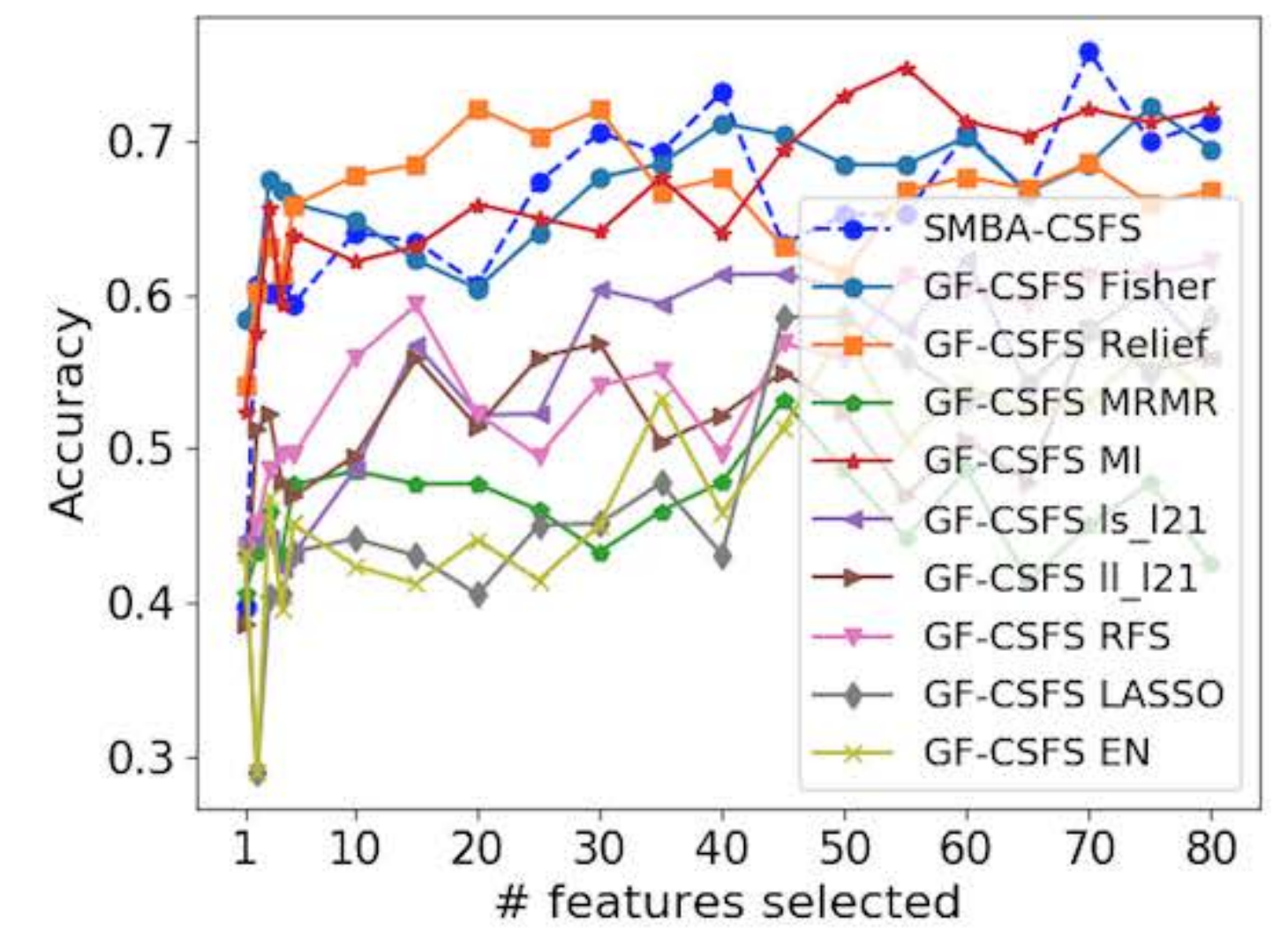
(c) CLL_SUB_111 (3)
