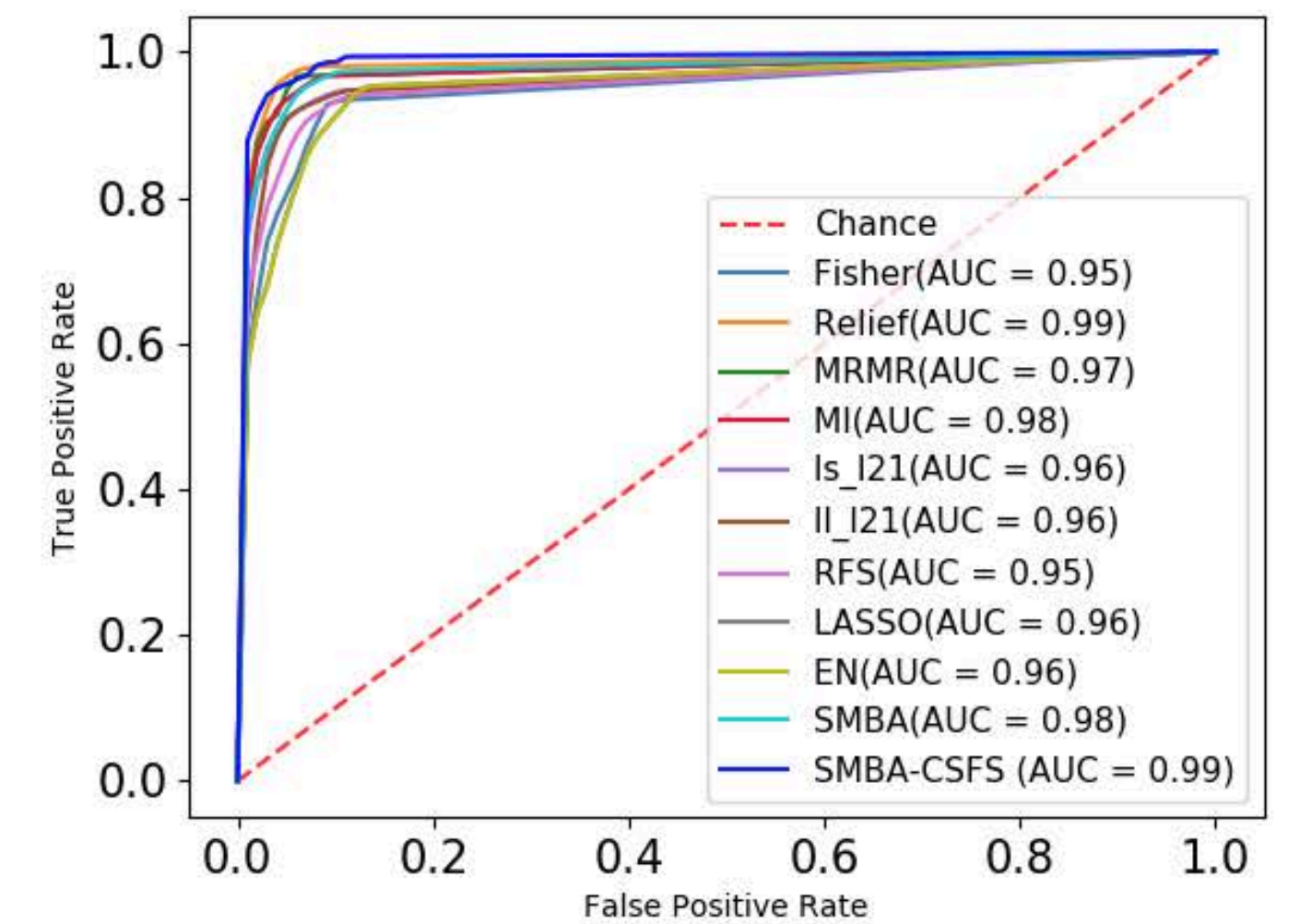
(i) GCM (14)
