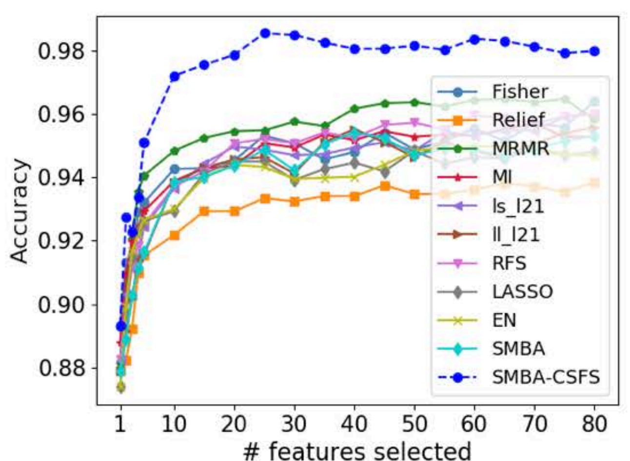
(i) GCM (14)
