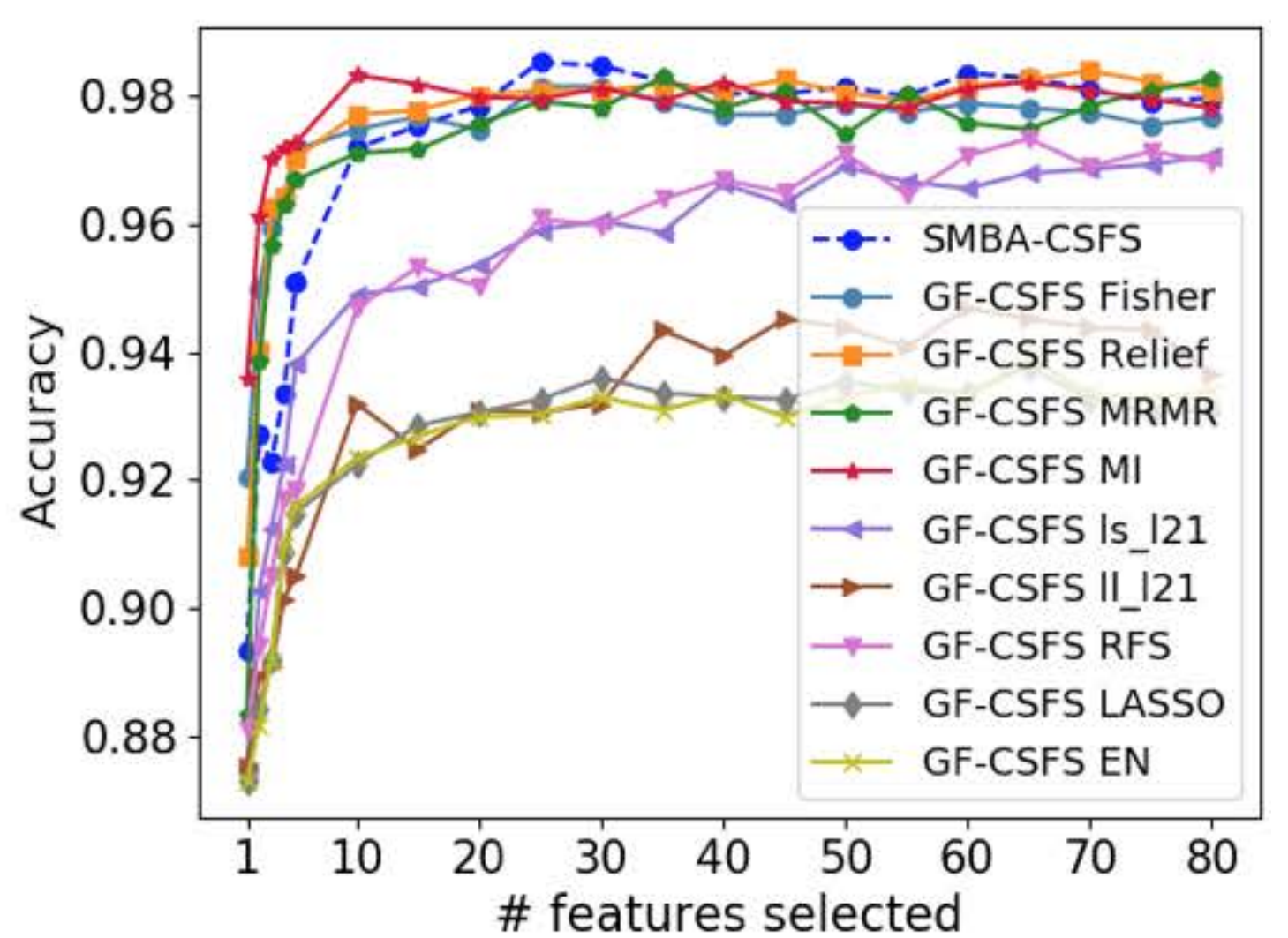
(i) GCM (14)
