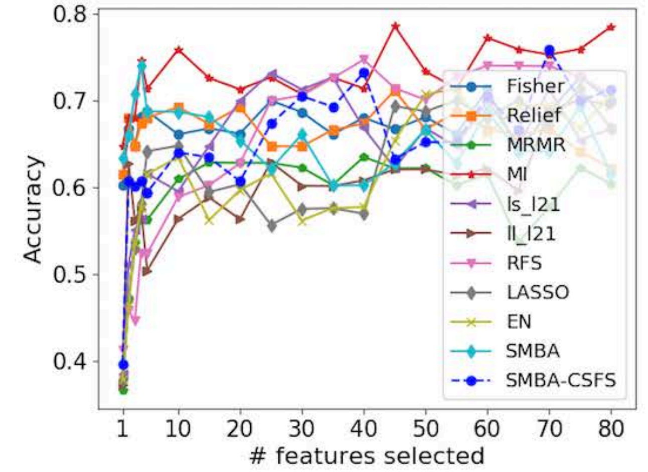
(c) CLL_SUB_111 (3)
