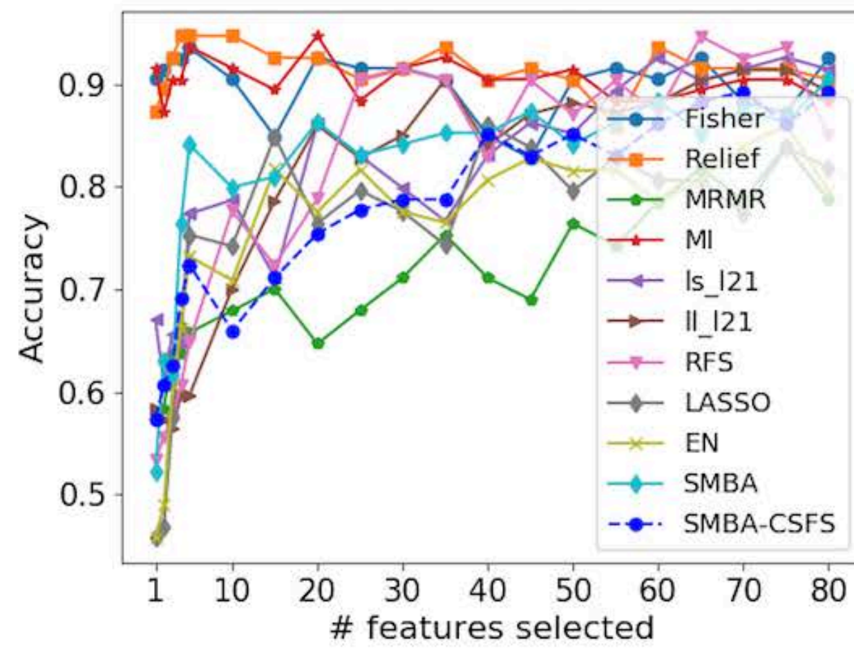
(a) ALLAML (2)
