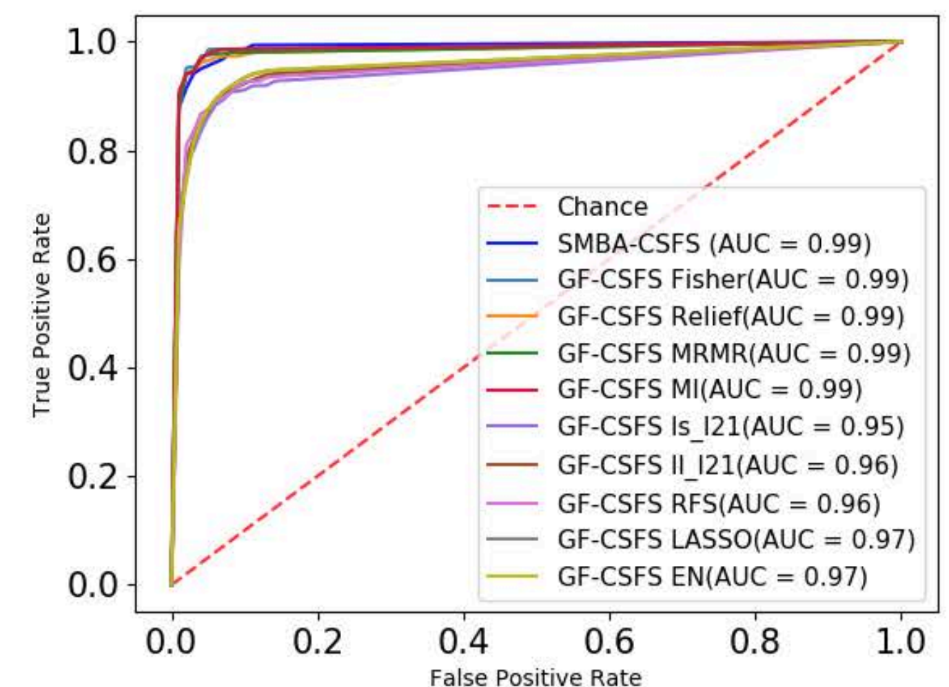
(i) GCM (14)
