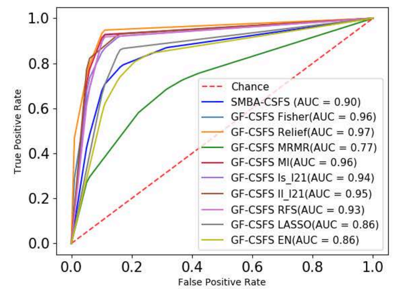
(c) CLL_SUB_111 (3)
