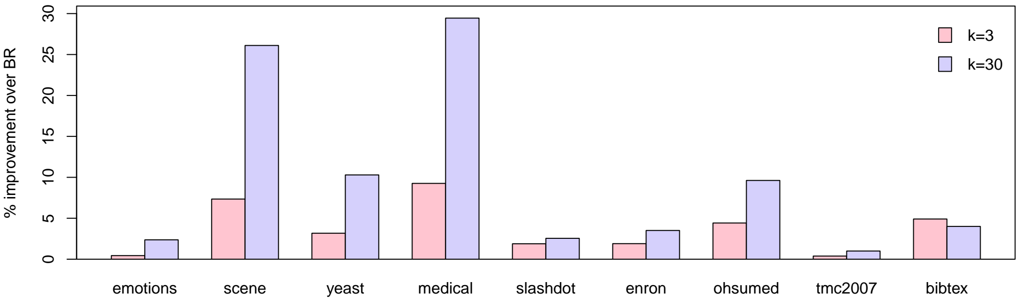
0/1 loss
