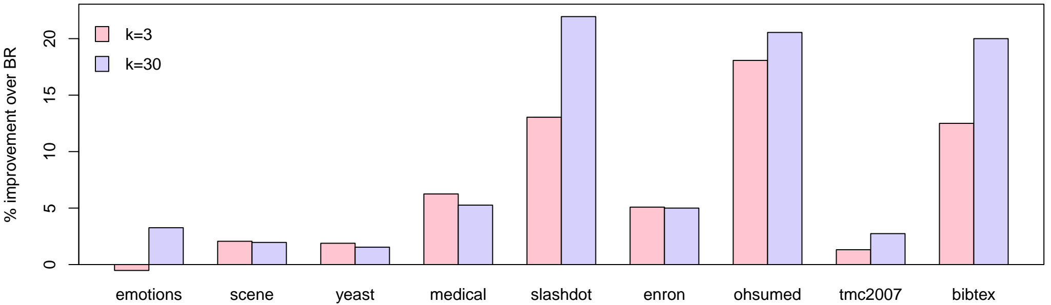
Hamming loss
