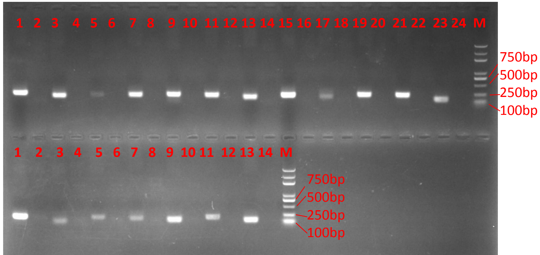
Figure S4: Odd number lane mean PCR amplification Include template; even numbers lane mean no template PCR. First row: Lane1-2: GRMZM2G024887 ; Lane3-4: GRMZM2G072448 ; Lane5-6; GRMZM2G300969 ; Lane7-8; GRMZM2G347047 ; Lane9-10: GRMZM2G390678 ; Lane11-12; GRMZM2G401874 ; Lane13-14; GRMZM2G419452 ; Lane15-16; GRMZM2G454608 ; Lane17-18: GRMZM2G045030 ; Lane19-20; GRMZM2G109973 ; Lane21-22; GRMZM2G339781 ; Lane13-14; GRMZM2G435294 . Seconed row: Lane1-2: AC209946.4-FG001 ; Lane3-4: GRMZM2G020761 ; Lane5-6; GRMZM2G024680 ; Lane7- 8; GRMZM2G127418 ; Lane9-10: GRMZM2G322493 ; Lane11-12; GRMZM2G457789 ; Lane13-14; LOC100282267
