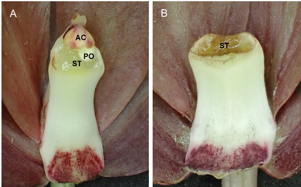
Figure S1 Column morphology of Eulophia zollingeri flowers in Ogimi-son, Okinawa, Japan. (A) Column with a degenerate rostellum, which facilitates autogamy. (B) Column with neither a rostellum nor anther cap and pollinaria. AC, anther cap; PO, pollinaria; ST, stigma.
