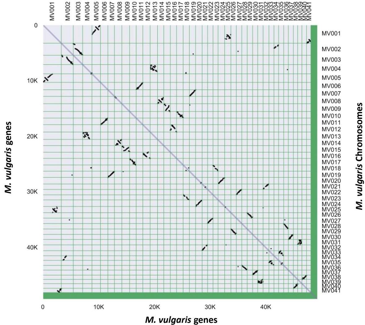
Figure S4. Intra-genomic comparison within M. vulgaris by 6,453 gene pairs.
