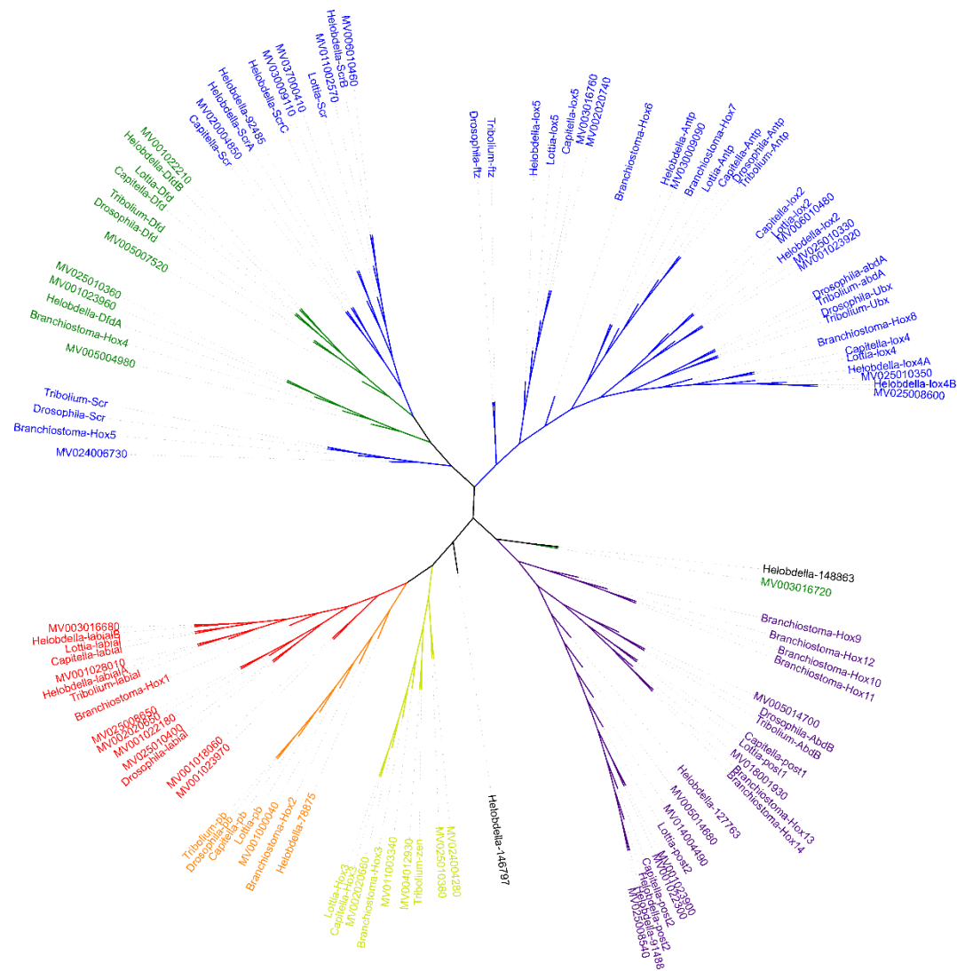
Figure S5. Forty one Hox genes identified in M. vulgaris genome, along with the Hox genes from spiralian genomes. Red, orange, yellow, green, blue, purple were assigned to paralog groups (Hox1, Hox2, Hox3, Hox4, central class and posterior class). MV003016720 in green belonged to Hox4, which was based on the BLASTP hits to NR (Non-Redundant Protein Sequence Database).
