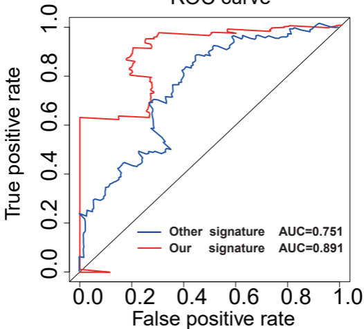
ROC curve
