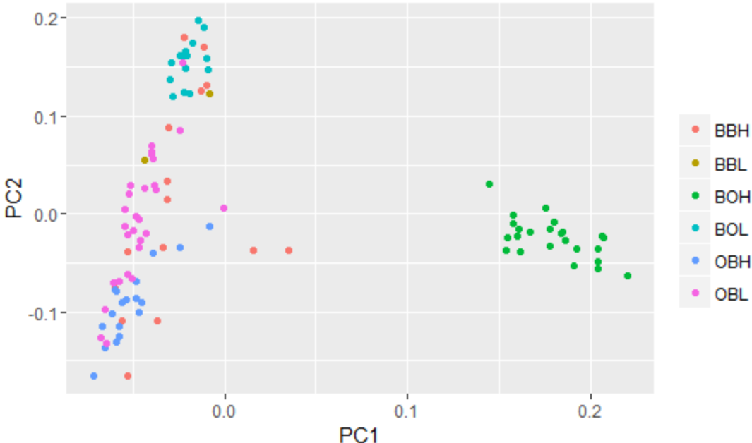
Projection onto PC1 and PC2
