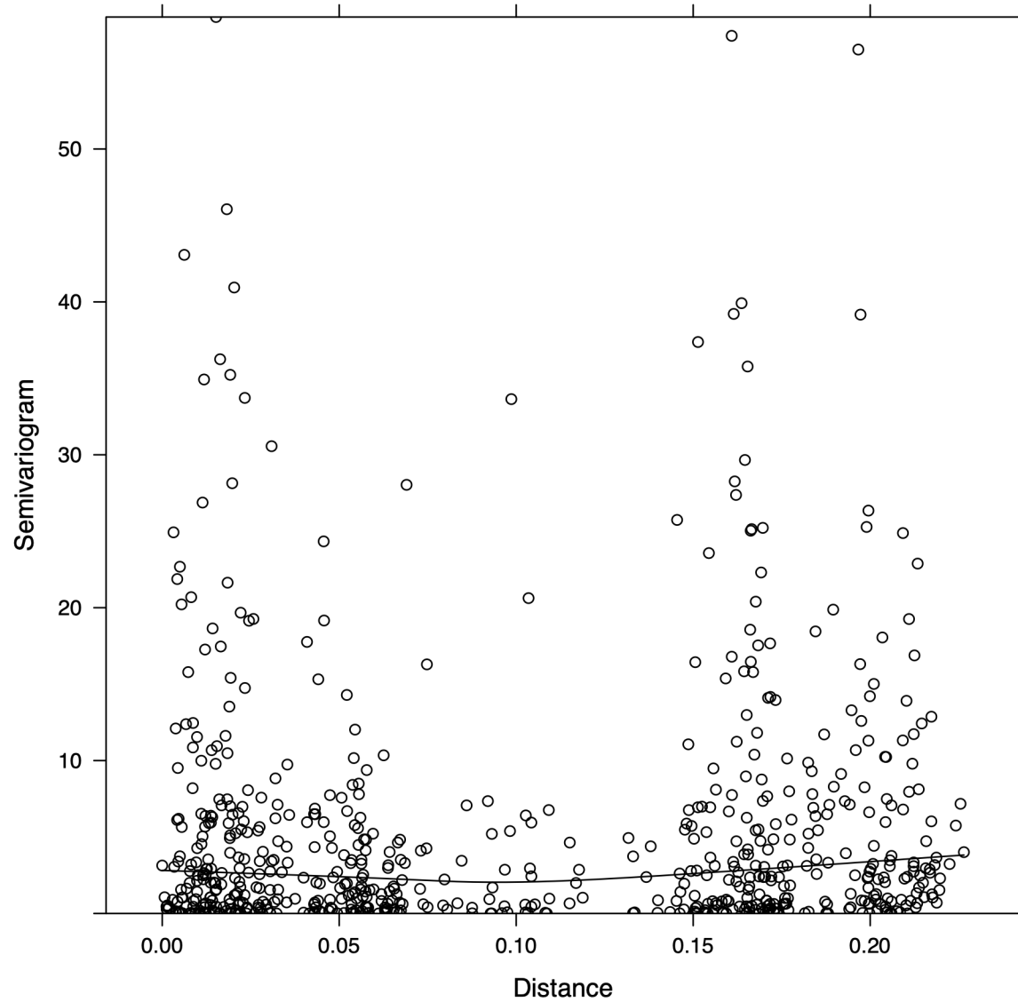
Variogram of residuals from the SEM. The plot shows no evidence for spatially auto-correlated residuals, indicating samples from same lakes can be treated as independent.
