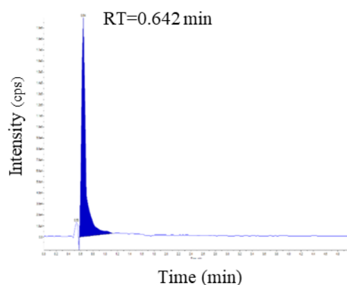
(C) 18:0 LPA
