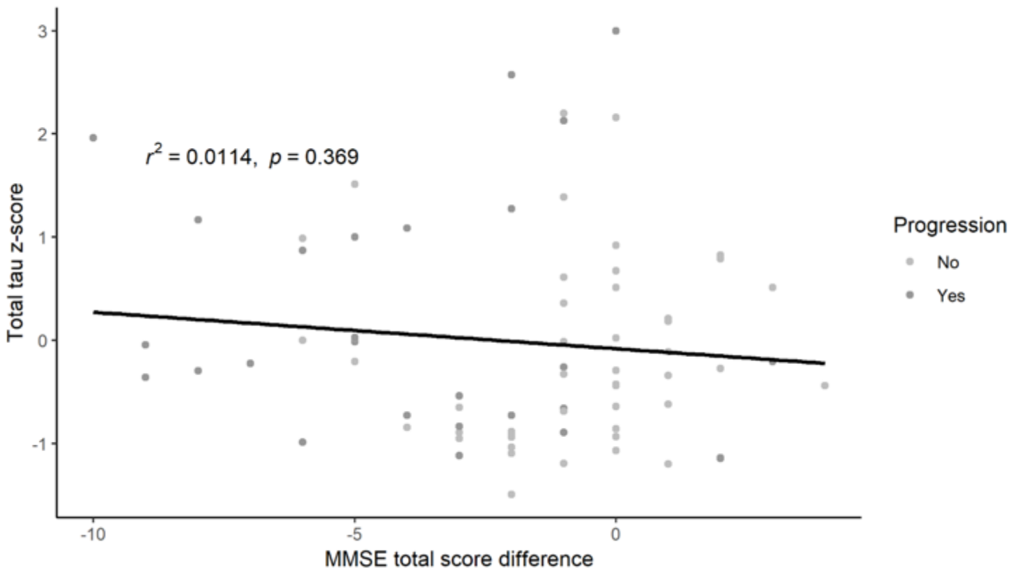
Total tau z-score vs. MMSE difference
