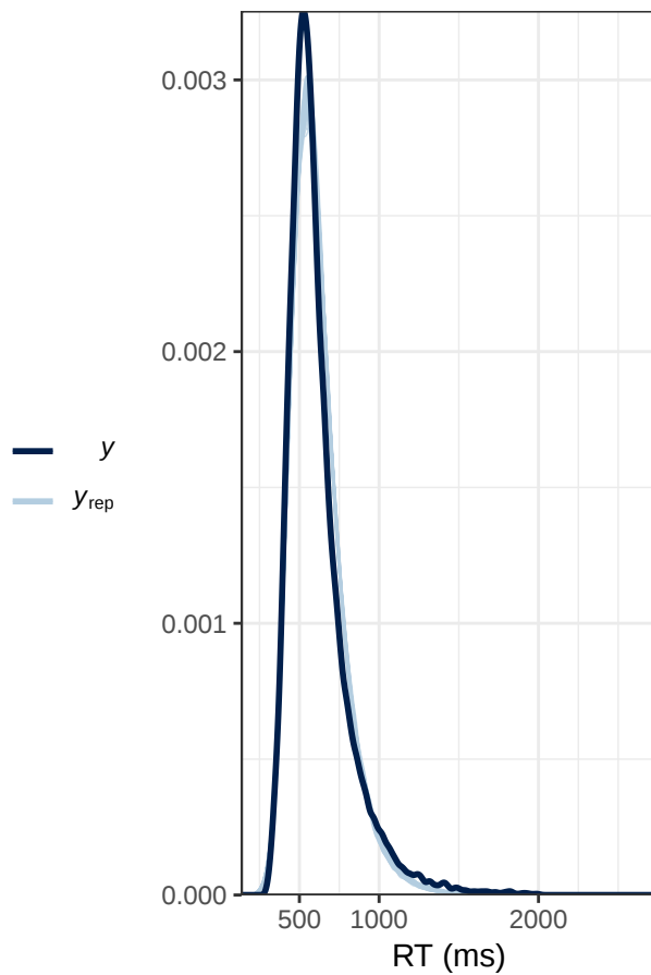
ExGaussian OLIFE
