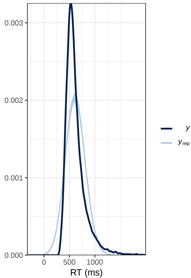
Gaussian SPQ
