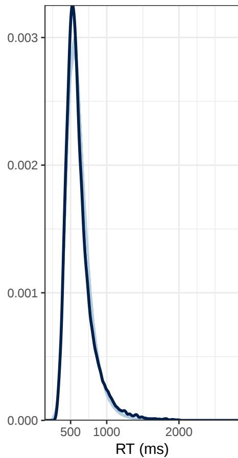
ExGaussian SPQ
