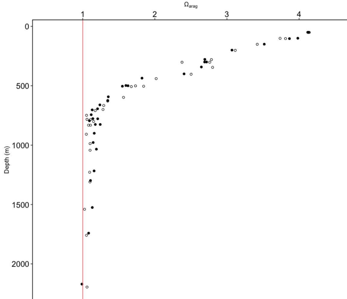
Supplementary Figure 1: Aragonite saturation state profiles for the Anegada Passage using measured (closed circle) and model predicted (open circle) \Omega_{\text{arag}} values (see Supplementary Table 1). A solid red vertical line at \Omega_{\text{arag}} = 1 represents the aragonite saturation horizon.
