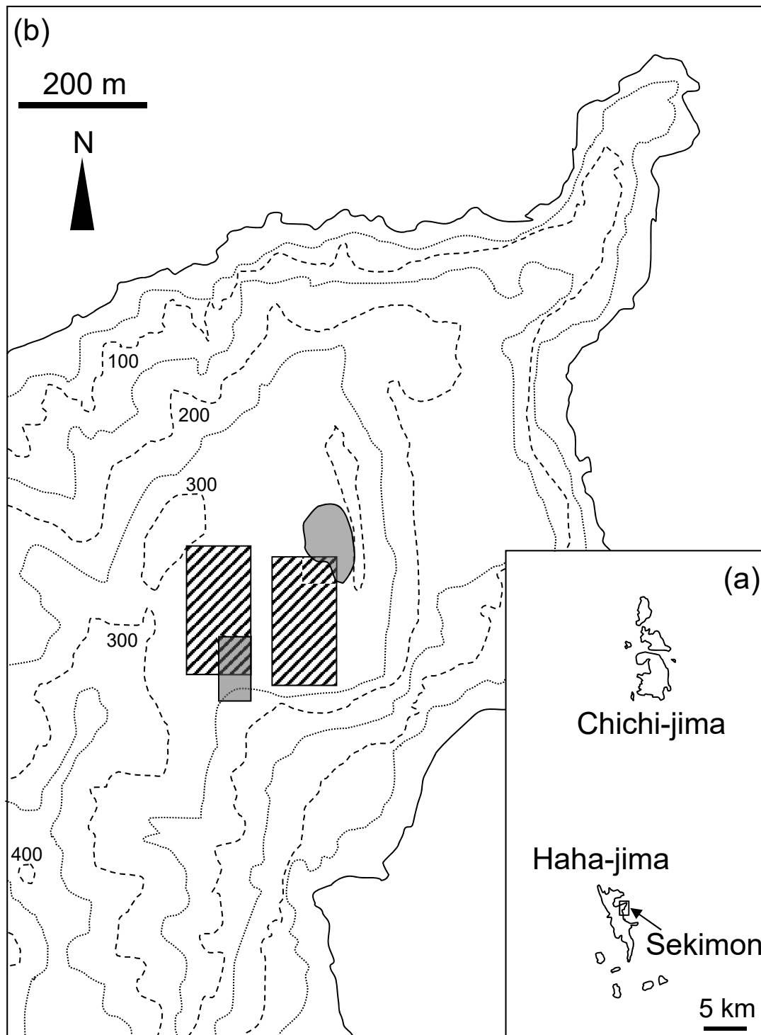
Fig. S1 Location of study site. (a) Haha-jima Island and the Sekimon forests on uplifted limestone and (b) the census plots in the Sekimon forests. Crosshatched rectangles are the two 2-ha plots surveyed in the present study; the gray-shaded rectangle at the southern edge of the western plot represents the plot studied by Shimizu (1994), of which the southernmost part was lost to a landslide. the irregular gray-shaded area at the northeastern corner of the eastern plot represents a former Bischofia javanica plantation.
