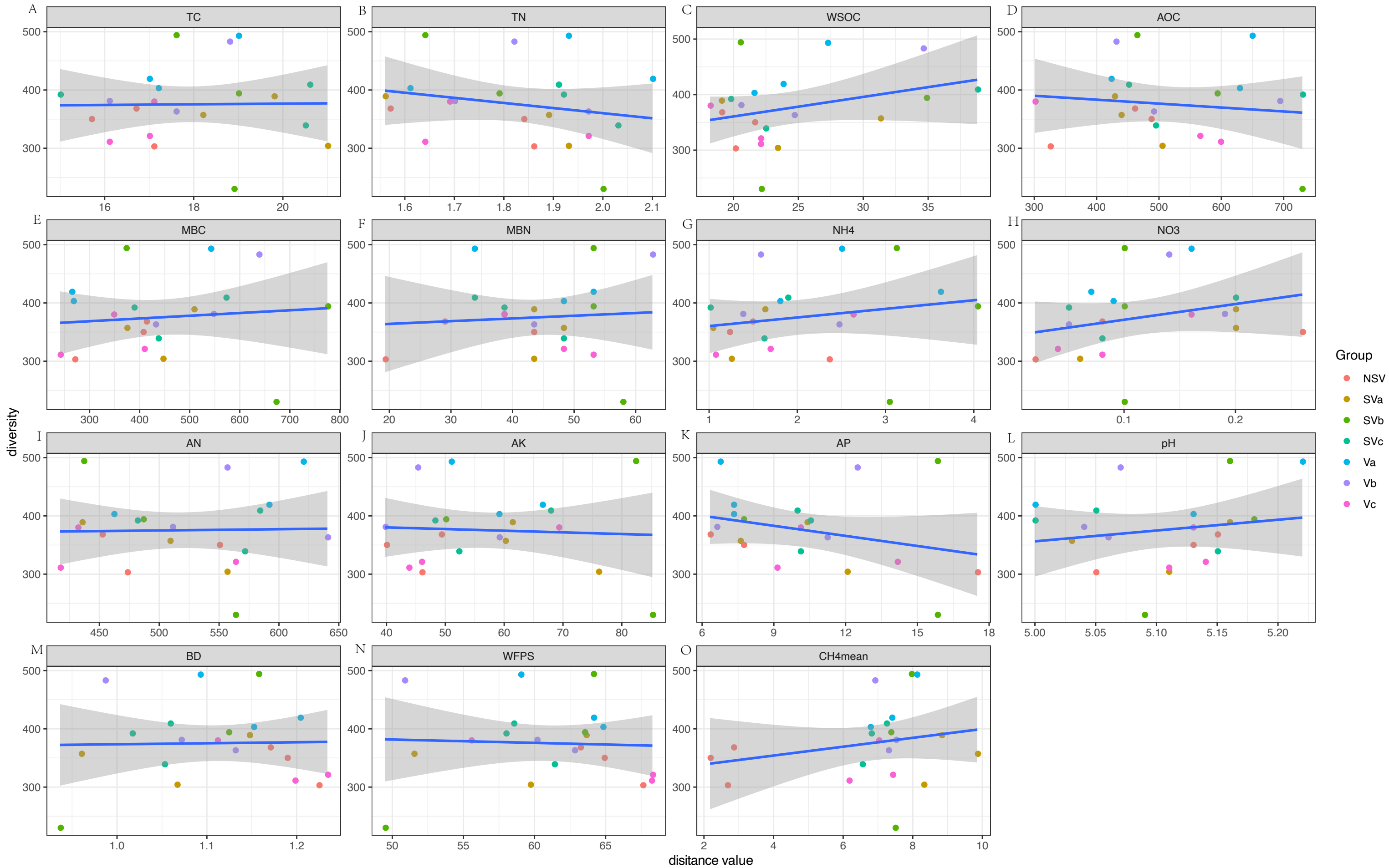
S Fig. 2 The relations between fungal community and environmental factors. S, straw; V, vetch; a = 0, b = 15, c = 30 kg ha -1 N from vetch; NSV, no straw or vetch. TC, total carbon; TN, total nitrogen; AOC, activated organic carbon; MBC, microbial biomass carbon; MBN, microbial biomass nitrogen; NH 4 -N, ammonium nitrogen; NO 3 -N, nitrate nitrogen; AN, alkali-hydrolysable nitrogen; AK, available potassium; AP, available phosphorus; BD, bulk density; WFPS, water-filled pore space; CH 4 mean, cumulative emission of methane in the early rice season(from pot experiment); .
