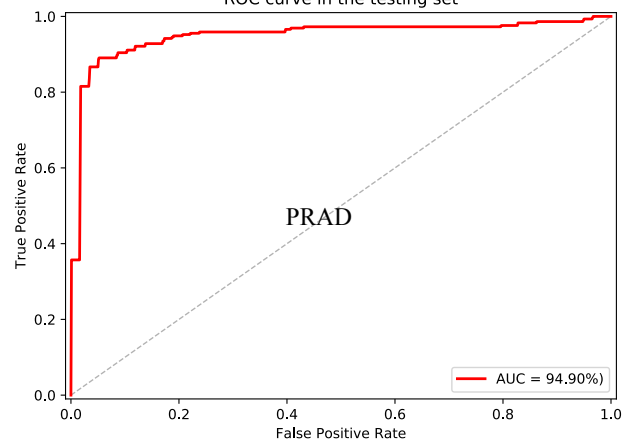
ROC curve in the testing set
