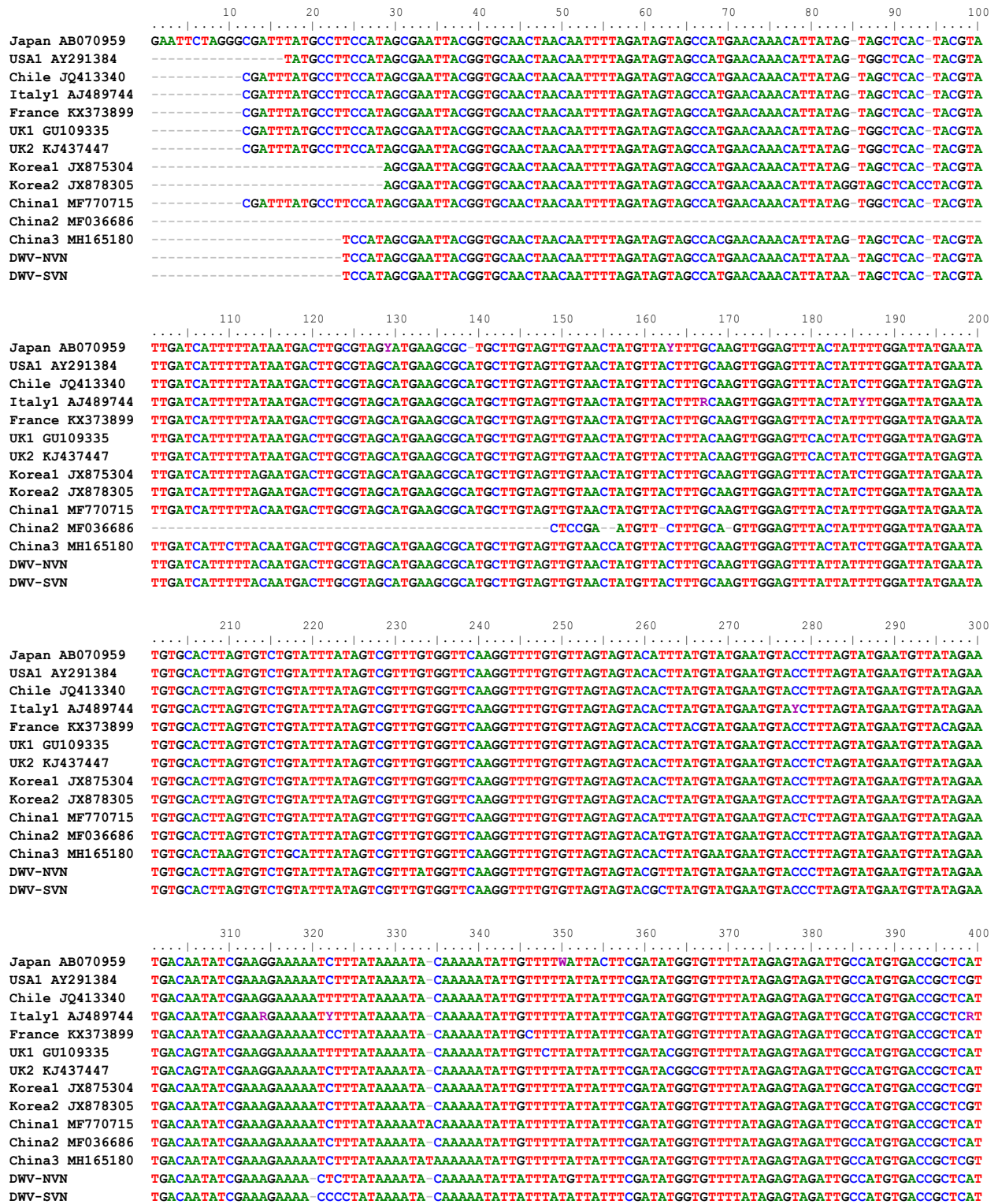
Fig. S2. Multiple alignment sequence of complete genome sequence of DWV strains in this study.
